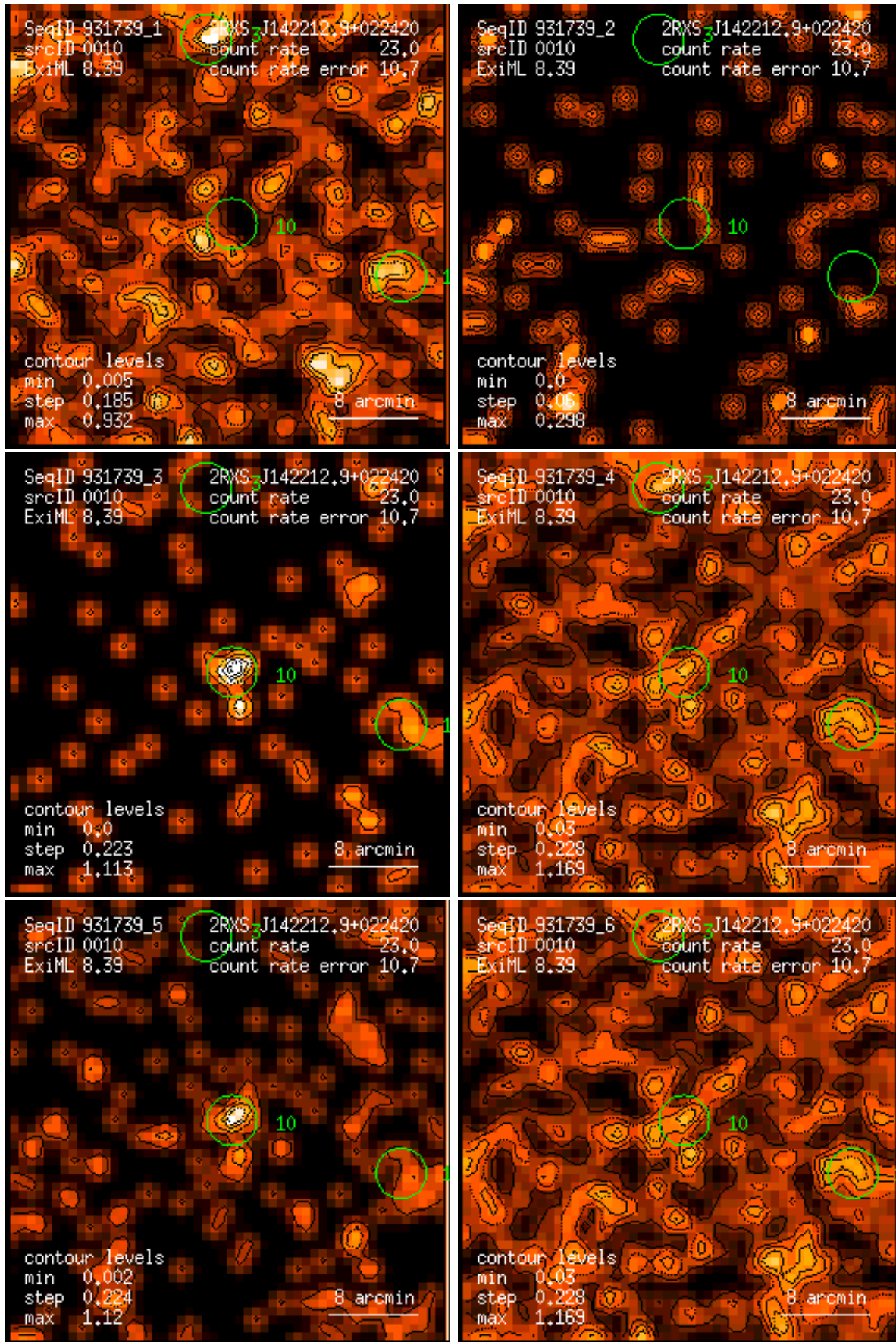
Figure 10: RASS 931739: detection 0010: band rate images, Gaussian filter: (1) PSPC channels 11 – 41, (2) 52 – 90, (3) 91 – 201, (4) 11 – 235, (5) 52 – 201, (6) 11 – 201. Broad band rates in counts/ks. Band rate contour levels in counts/ks/arcmin 2 .
