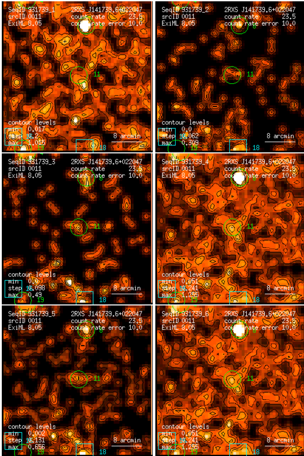
Figure 11: RASS 931739: detection 0011: band rate images, Gaussian filter: (1) PSPC channels 11 – 41, (2) 52 – 90, (3) 91 – 201, (4) 11 – 235, (5) 52 – 201, (6) 11 – 201. Broad band rates in counts/ks. Band rate contour levels in counts/ks/arcmin 2 .
