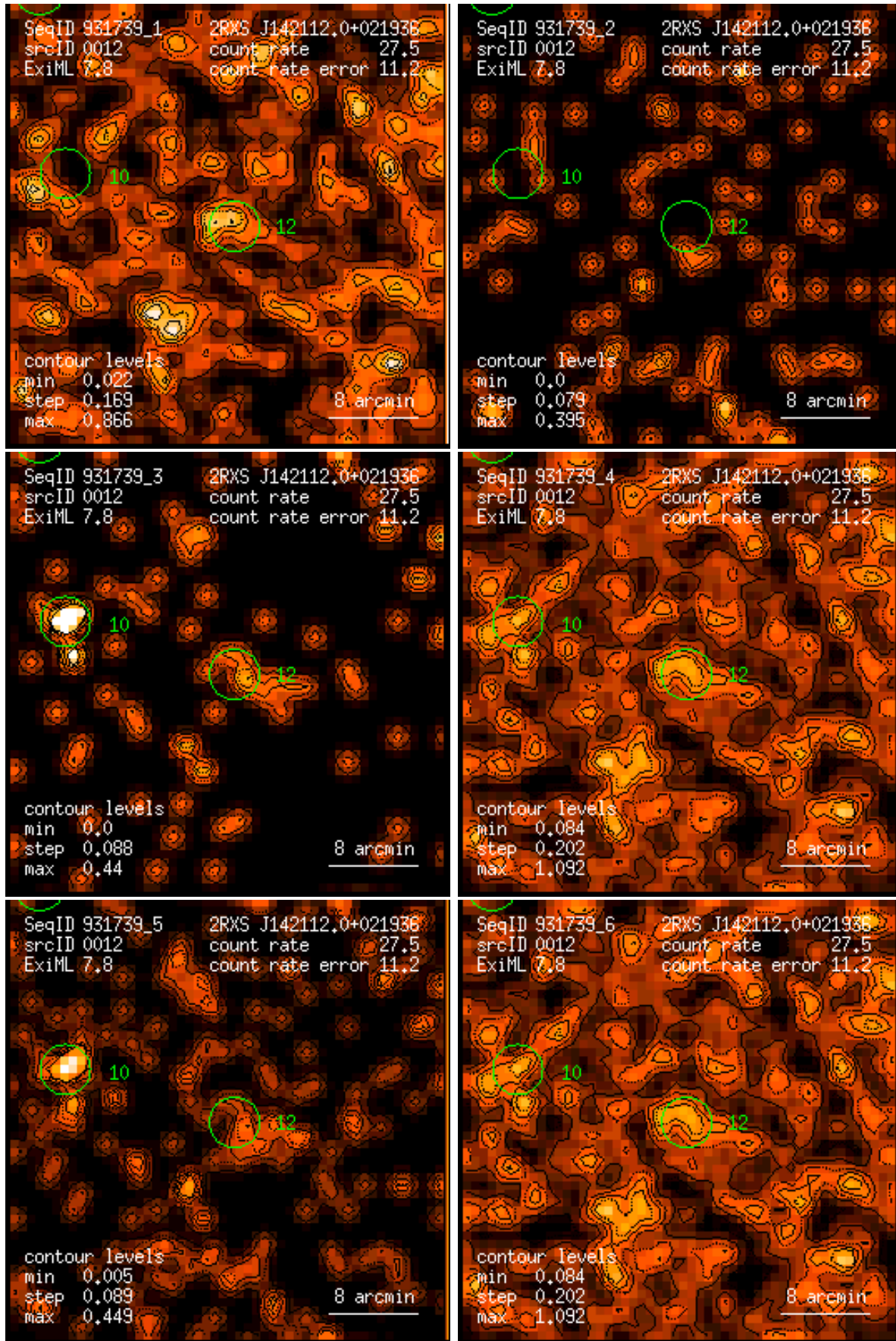
Figure 12: RASS 931739: detection 0012: band rate images, Gaussian filter: (1) PSPC channels 11 – 41, (2) 52 – 90, (3) 91 – 201, (4) 11 – 235, (5) 52 – 201, (6) 11 – 201. Broad band rates in counts/ks. Band rate contour levels in counts/ks/arcmin 2 .
