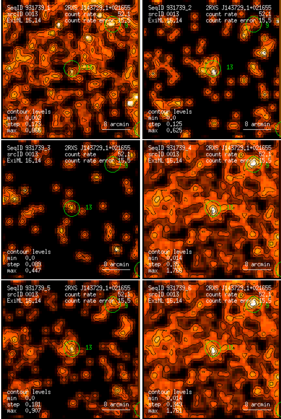
Figure 13: RASS 931739: detection 0013: band rate images, Gaussian filter: (1) PSPC channels 11 – 41, (2) 52 – 90, (3) 91 – 201, (4) 11 – 235, (5) 52 – 201, (6) 11 – 201. Broad band rates in counts/ks. Band rate contour levels in counts/ks/arcmin 2 .
