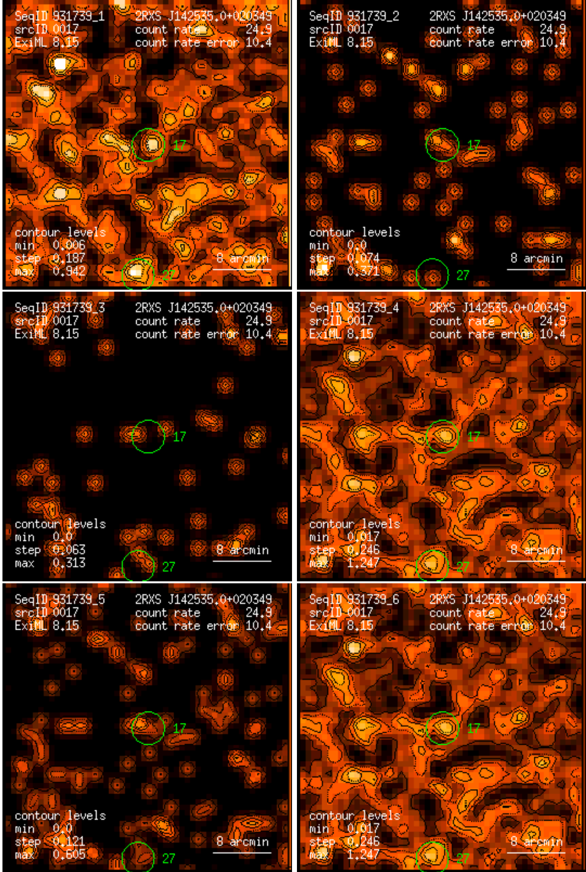
Figure 17: RASS 931739: detection 0017: band rate images, Gaussian filter: (1) PSPC channels 11 – 41, (2) 52 – 90, (3) 91 – 201, (4) 11 – 235, (5) 52 – 201, (6) 11 – 201. Broad band rates in counts/ks. Band rate contour levels in counts/ks/arcmin 2 .
