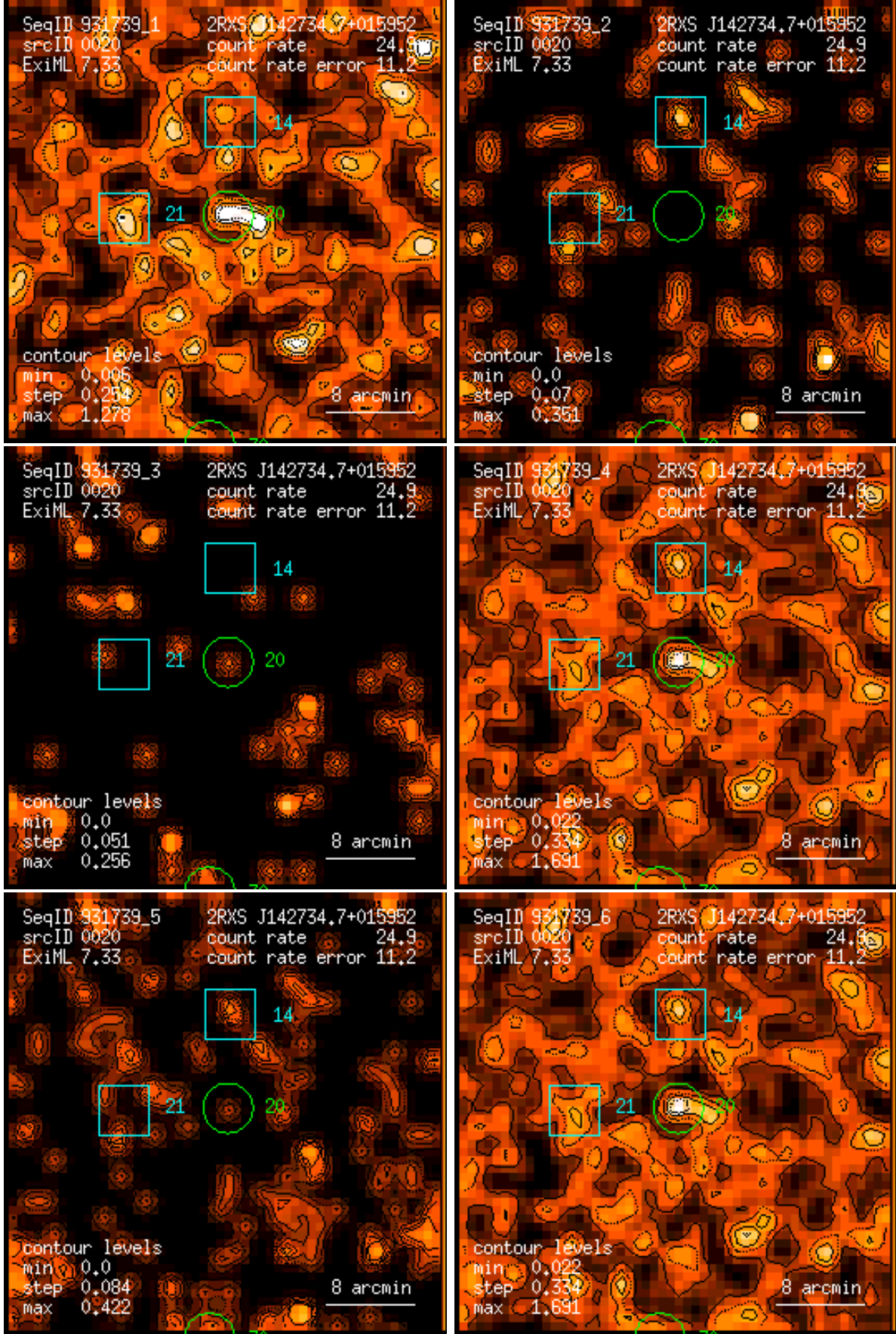
Figure 20: RASS 931739: detection 0020: band rate images, Gaussian filter: (1) PSPC channels 11 – 41, (2) 52 – 90, (3) 91 – 201, (4) 11 – 235, (5) 52 – 201, (6) 11 – 201. Broad band rates in counts/ks. Band rate contour levels in counts/ks/arcmin 2 .
