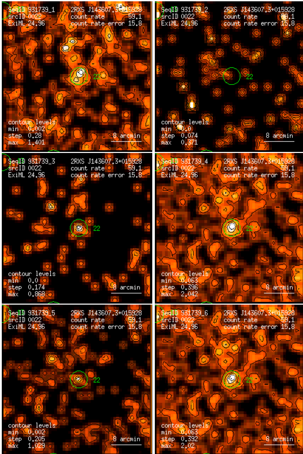
Figure 22: RASS 931739: detection 0022: band rate images, Gaussian filter: (1) PSPC channels 11 – 41, (2) 52 – 90, (3) 91 – 201, (4) 11 – 235, (5) 52 – 201, (6) 11 – 201. Broad band rates in counts/ks. Band rate contour levels in counts/ks/arcmin 2 .
