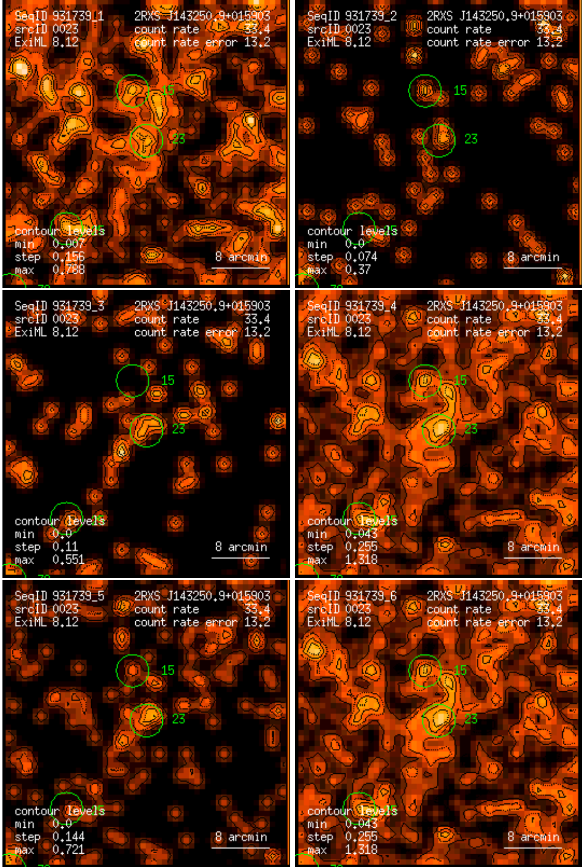
Figure 23: RASS 931739: detection 0023: band rate images, Gaussian filter: (1) PSPC channels 11 – 41, (2) 52 – 90, (3) 91 – 201, (4) 11 – 235, (5) 52 – 201, (6) 11 – 201. Broad band rates in counts/ks. Band rate contour levels in counts/ks/arcmin 2 .
