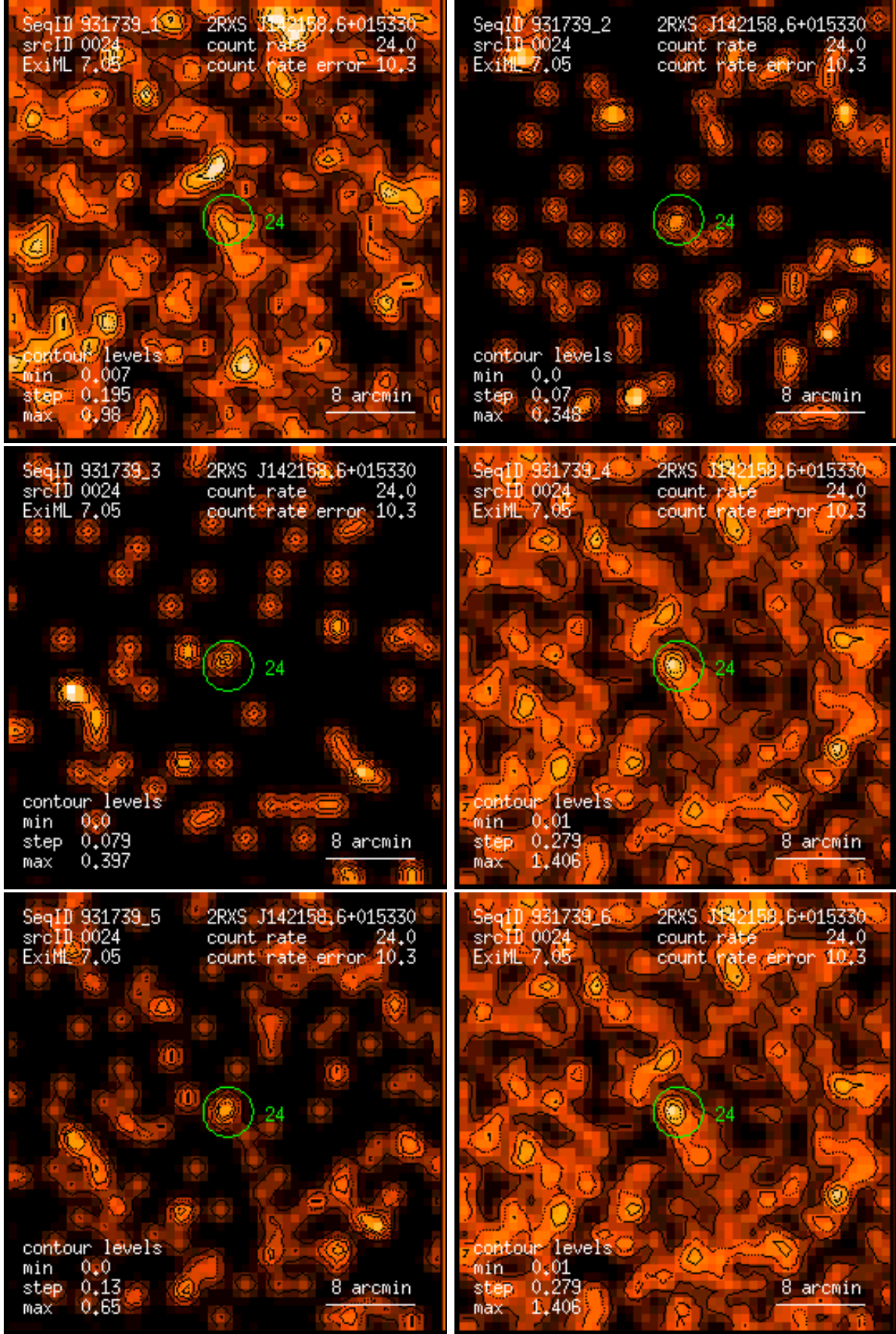
Figure 24: RASS 931739: detection 0024: band rate images, Gaussian filter: (1) PSPC channels 11 – 41, (2) 52 – 90, (3) 91 – 201, (4) 11 – 235, (5) 52 – 201, (6) 11 – 201. Broad band rates in counts/ks. Band rate contour levels in counts/ks/arcmin 2 .
