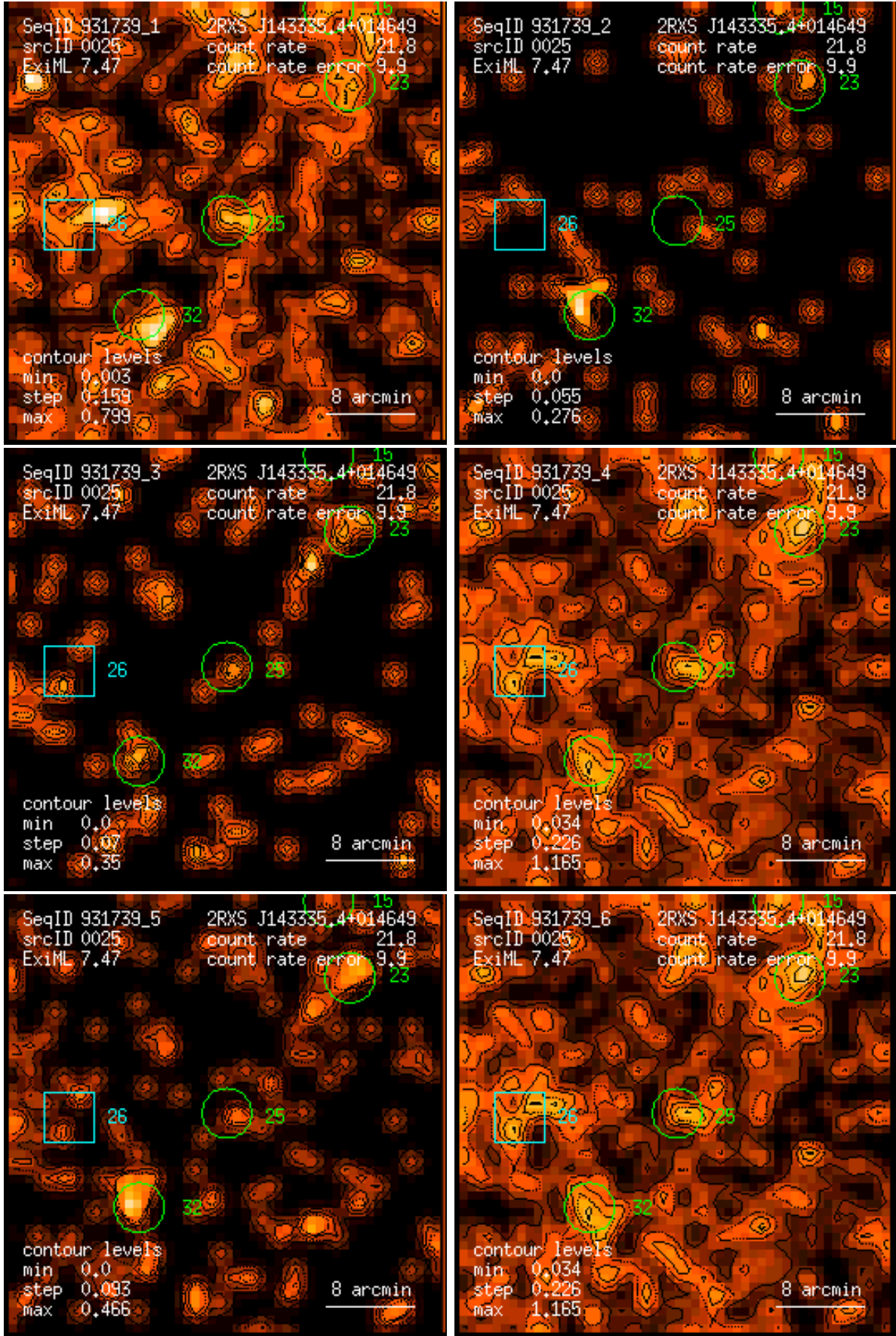
Figure 25: RASS 931739: detection 0025: band rate images, Gaussian filter: (1) PSPC channels 11 – 41, (2) 52 – 90, (3) 91 – 201, (4) 11 – 235, (5) 52 – 201, (6) 11 – 201. Broad band rates in counts/ks. Band rate contour levels in counts/ks/arcmin 2 .
