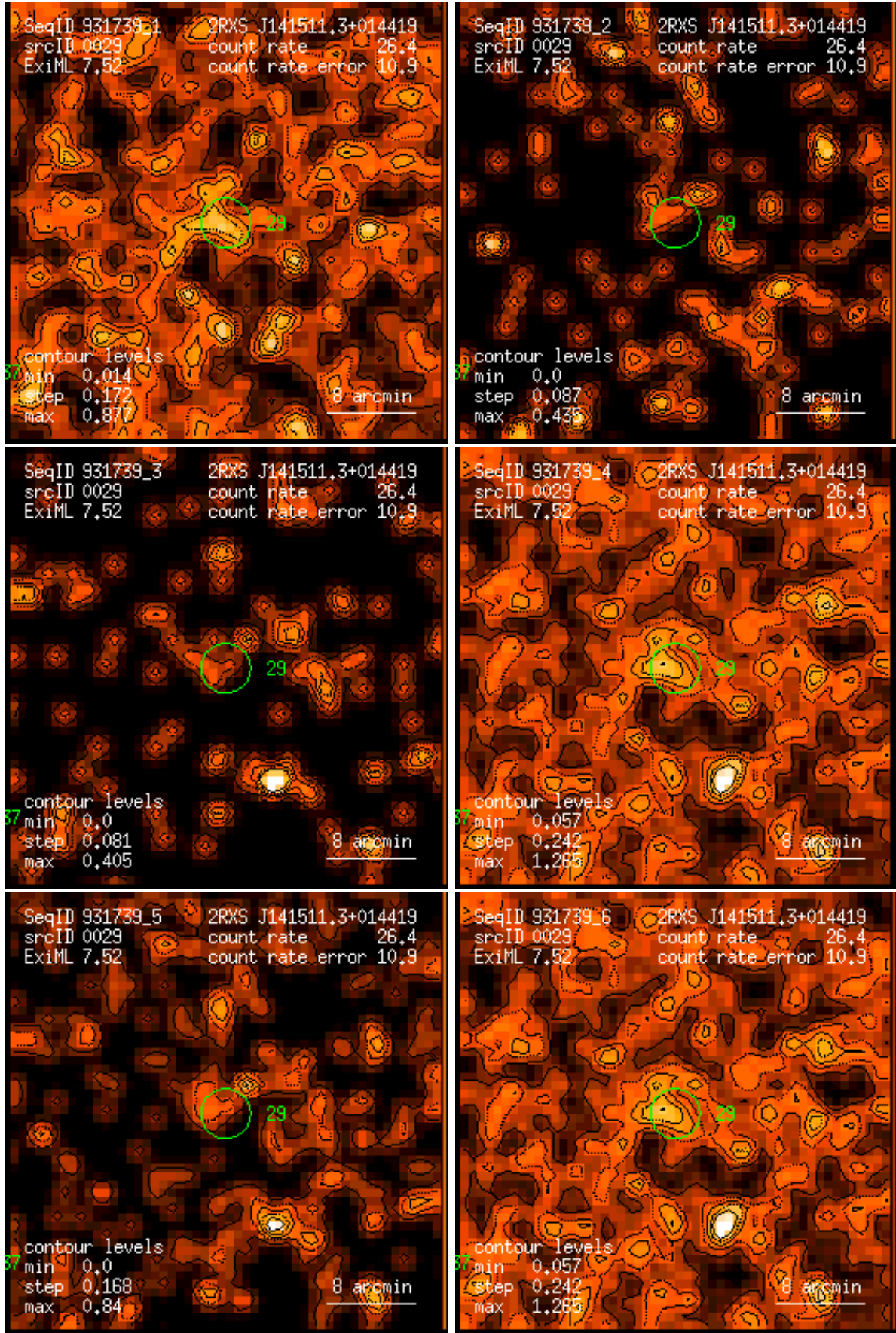
Figure 29: RASS 931739: detection 0029: band rate images, Gaussian filter: (1) PSPC channels 11 – 41, (2) 52 – 90, (3) 91 – 201, (4) 11 – 235, (5) 52 – 201, (6) 11 – 201. Broad band rates in counts/ks. Band rate contour levels in counts/ks/arcmin 2 .
