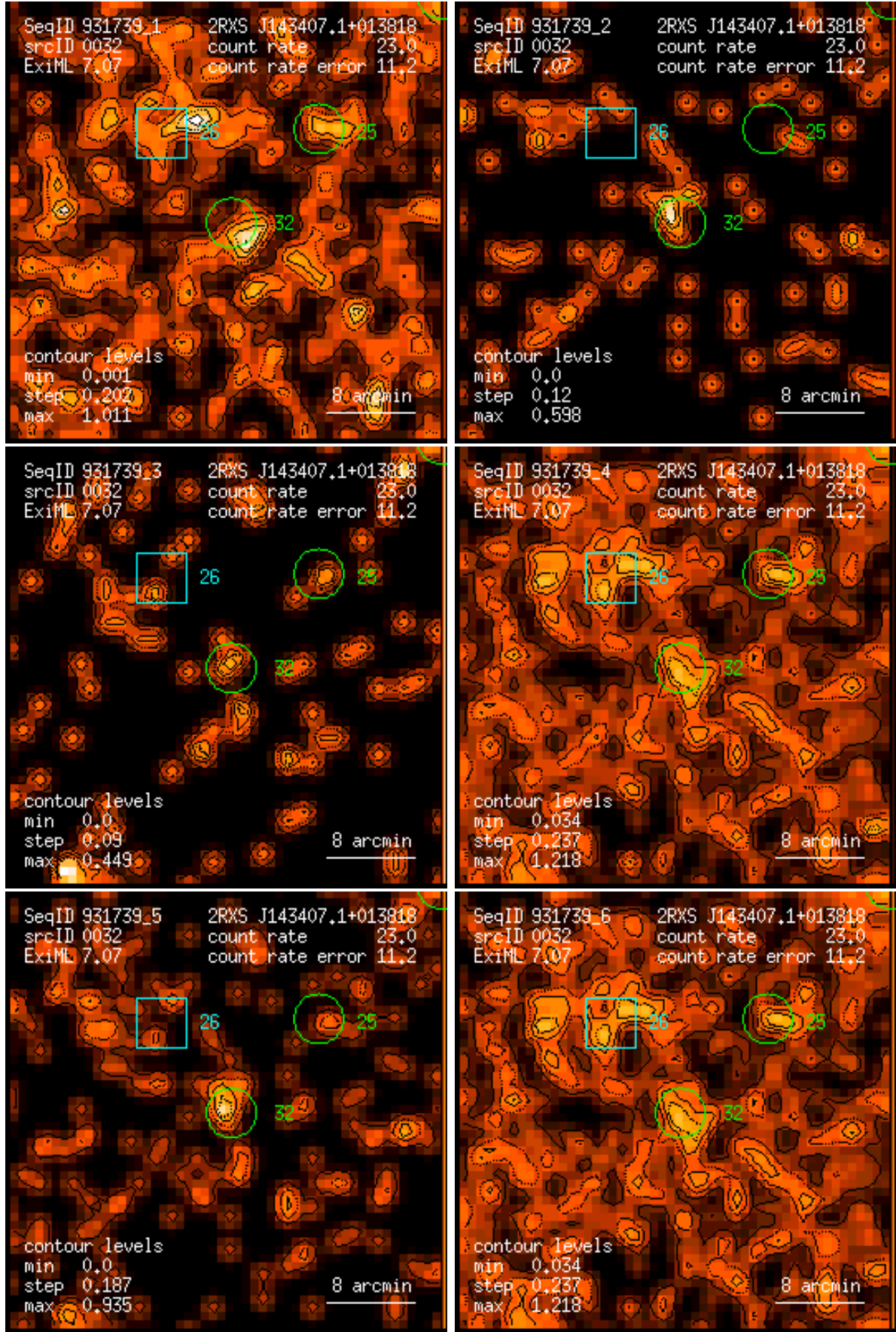
Figure 32: RASS 931739: detection 0032: band rate images, Gaussian filter: (1) PSPC channels 11 – 41, (2) 52 – 90, (3) 91 – 201, (4) 11 – 235, (5) 52 – 201, (6) 11 – 201. Broad band rates in counts/ks. Band rate contour levels in counts/ks/arcmin 2 .
