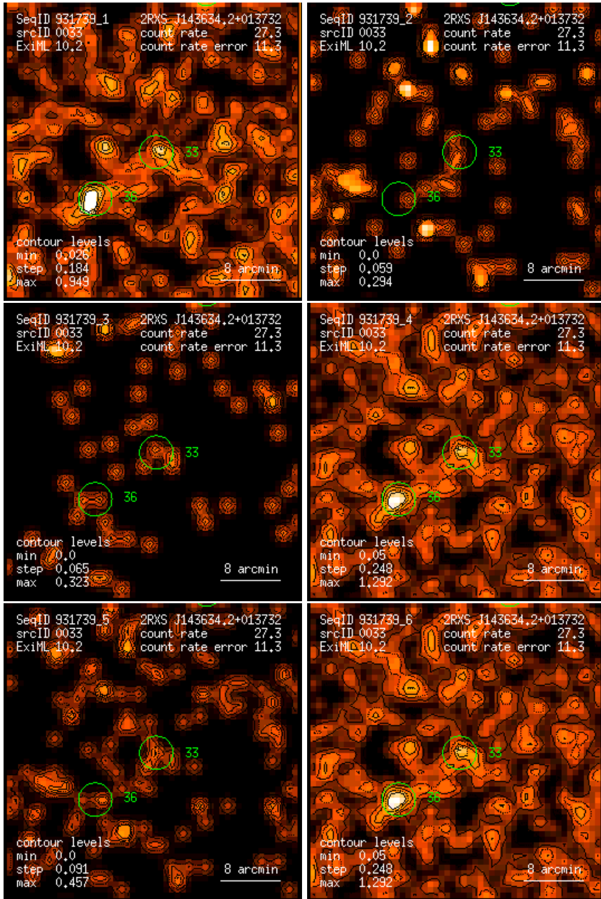
Figure 33: RASS 931739: detection 0033: band rate images, Gaussian filter: (1) PSPC channels 11 – 41, (2) 52 – 90, (3) 91 – 201, (4) 11 – 235, (5) 52 – 201, (6) 11 – 201. Broad band rates in counts/ks. Band rate contour levels in counts/ks/arcmin 2 .
