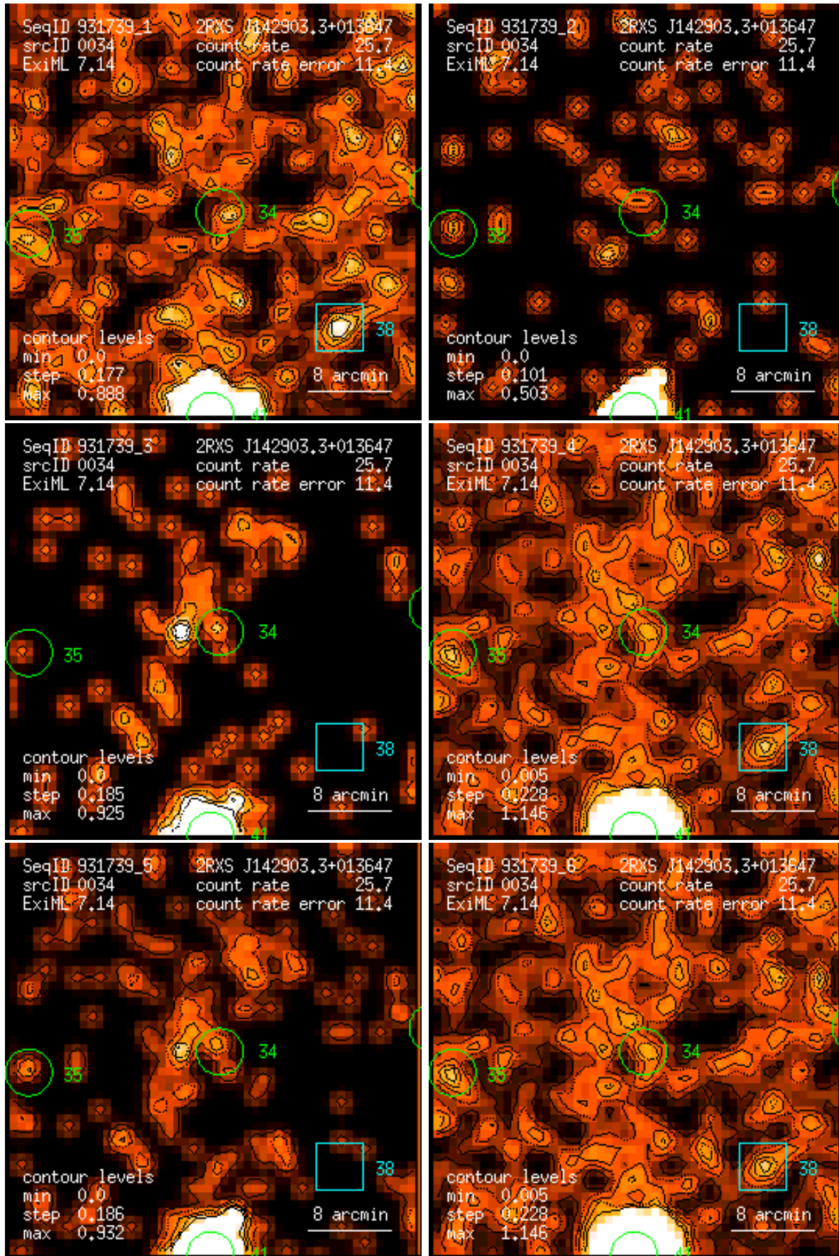
Figure 34: RASS 931739: detection 0034: band rate images, Gaussian filter: (1) PSPC channels 11 – 41, (2) 52 – 90, (3) 91 – 201, (4) 11 – 235, (5) 52 – 201, (6) 11 – 201. Broad band rates in counts/ks. Band rate contour levels in counts/ks/arcmin 2 .
