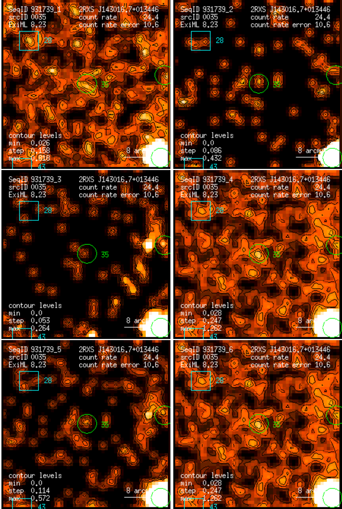
Figure 35: RASS 931739: detection 0035: band rate images, Gaussian filter: (1) PSPC channels 11 – 41, (2) 52 – 90, (3) 91 – 201, (4) 11 – 235, (5) 52 – 201, (6) 11 – 201. Broad band rates in counts/ks. Band rate contour levels in counts/ks/arcmin 2 .
