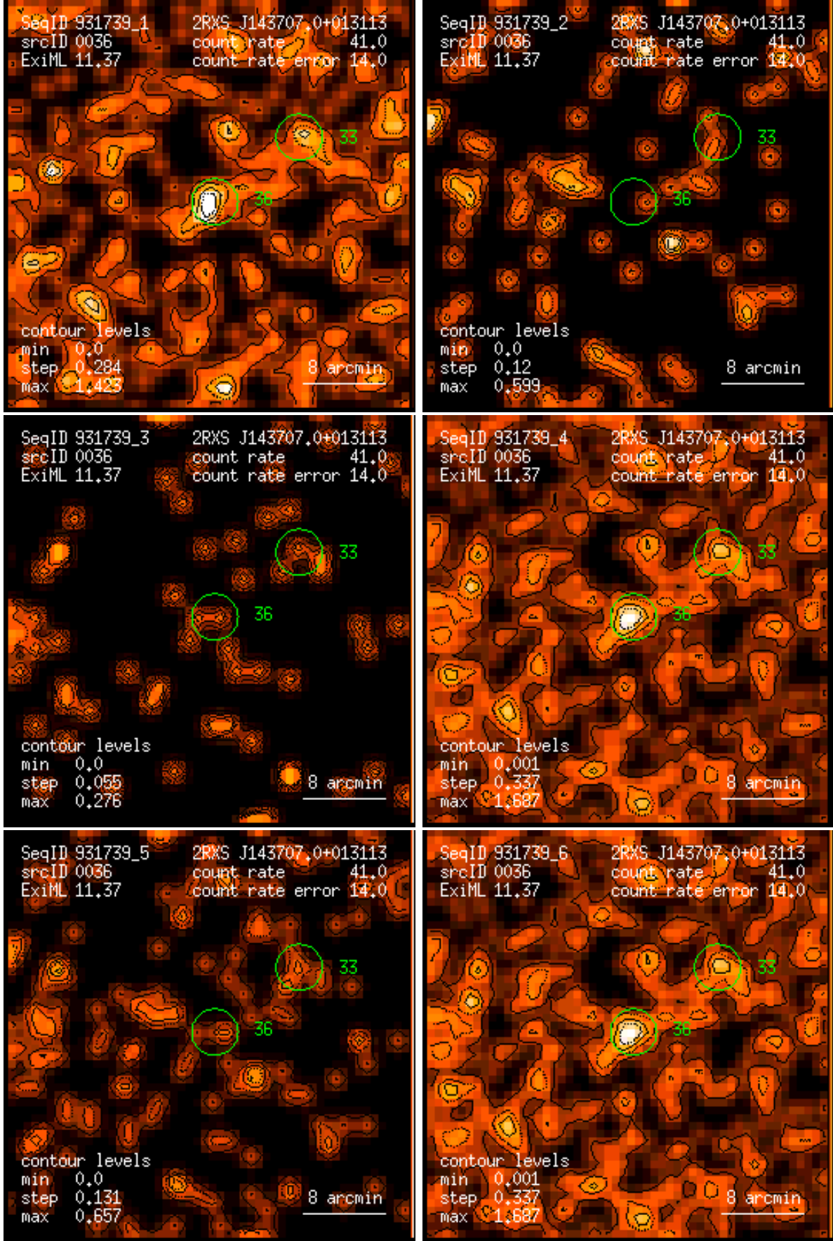
Figure 36: RASS 931739: detection 0036: band rate images, Gaussian filter: (1) PSPC channels 11 – 41, (2) 52 – 90, (3) 91 – 201, (4) 11 – 235, (5) 52 – 201, (6) 11 – 201. Broad band rates in counts/ks. Band rate contour levels in counts/ks/arcmin 2 .
