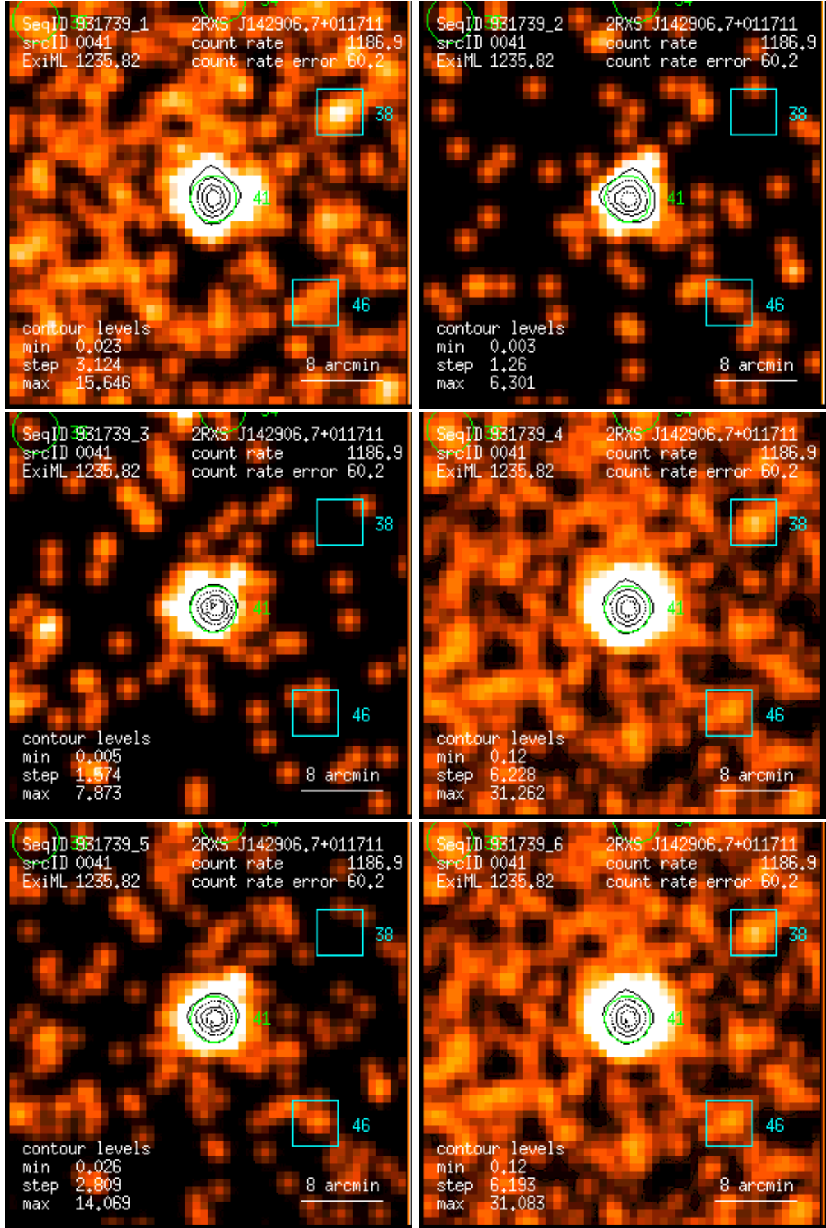
Figure 41: RASS 931739: detection 0041: band rate images, Gaussian filter: (1) PSPC channels 11 – 41, (2) 52 – 90, (3) 91 – 201, (4) 11 – 235, (5) 52 – 201, (6) 11 – 201. Broad band rates in counts/ks. Band rate contour levels in counts/ks/arcmin 2 .
