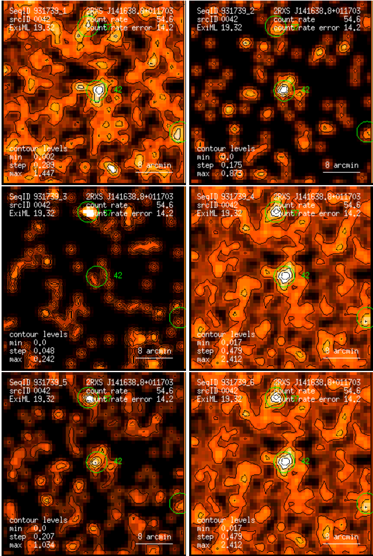
Figure 42: RASS 931739: detection 0042: band rate images, Gaussian filter: (1) PSPC channels 11 – 41, (2) 52 – 90, (3) 91 – 201, (4) 11 – 235, (5) 52 – 201, (6) 11 – 201. Broad band rates in counts/ks. Band rate contour levels in counts/ks/arcmin 2 .
