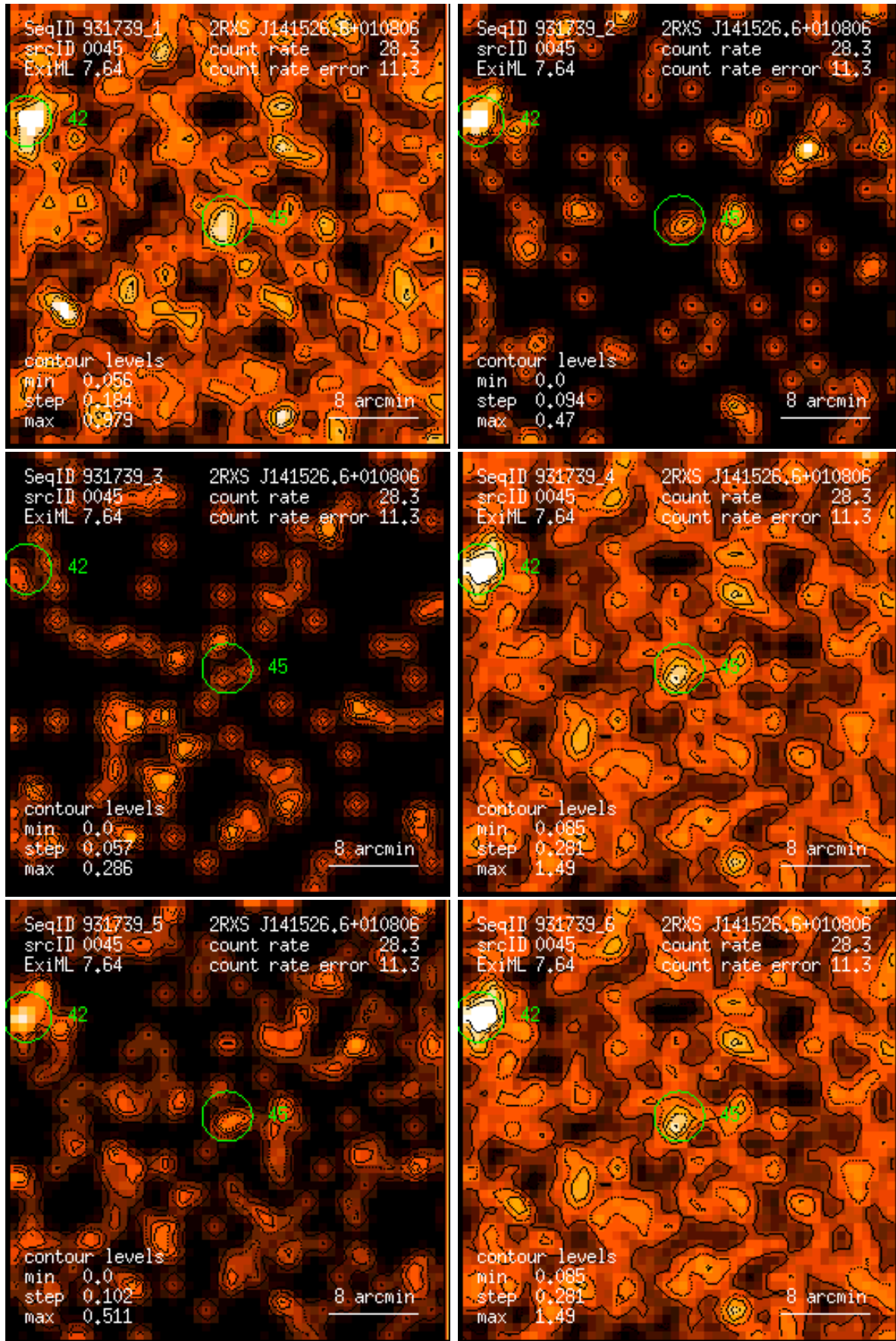
Figure 45: RASS 931739: detection 0045: band rate images, Gaussian filter: (1) PSPC channels 11 – 41, (2) 52 – 90, (3) 91 – 201, (4) 11 – 235, (5) 52 – 201, (6) 11 – 201. Broad band rates in counts/ks. Band rate contour levels in counts/ks/arcmin 2 .
