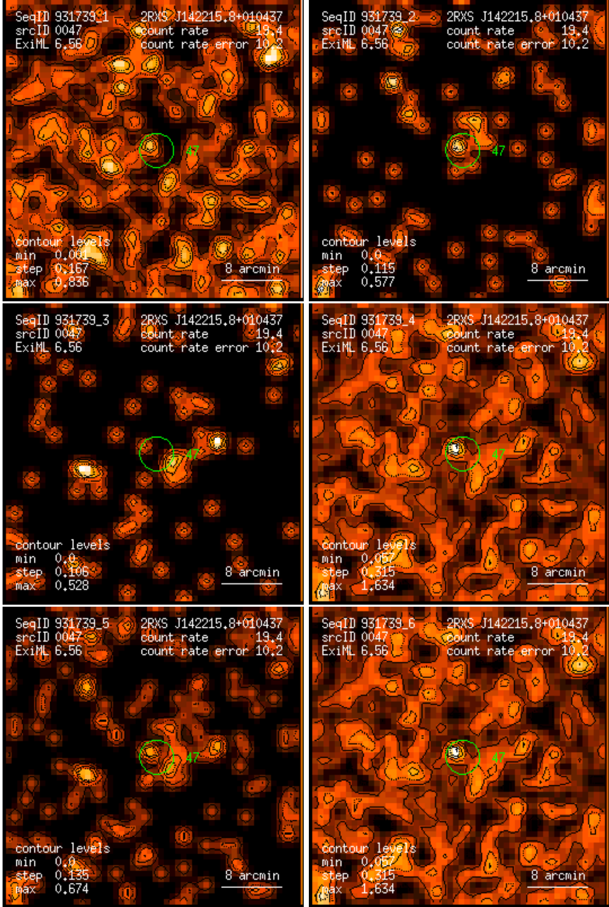
Figure 47: RASS 931739: detection 0047: band rate images, Gaussian filter: (1) PSPC channels 11 – 41, (2) 52 – 90, (3) 91 – 201, (4) 11 – 235, (5) 52 – 201, (6) 11 – 201. Broad band rates in counts/ks. Band rate contour levels in counts/ks/arcmin 2 .
