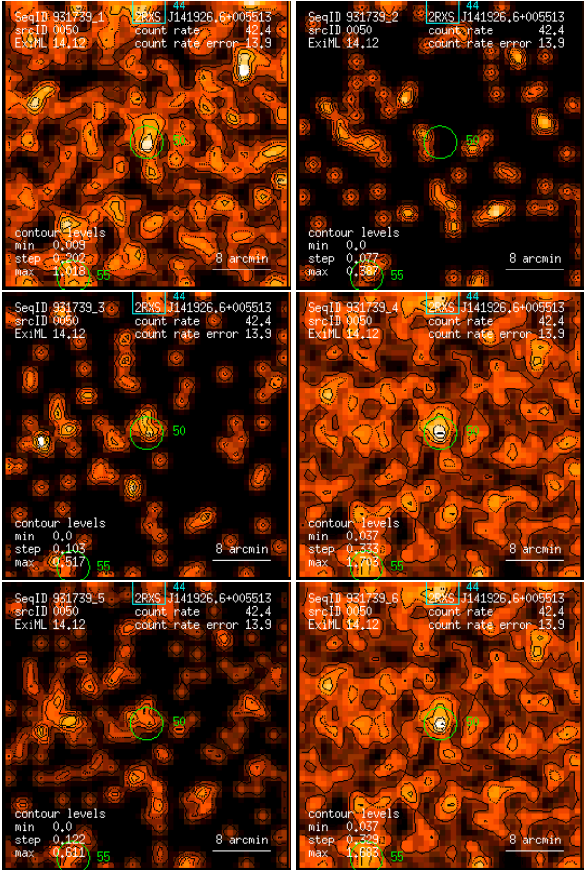
Figure 50: RASS 931739: detection 0050: band rate images, Gaussian filter: (1) PSPC channels 11 – 41, (2) 52 – 90, (3) 91 – 201, (4) 11 – 235, (5) 52 – 201, (6) 11 – 201. Broad band rates in counts/ks. Band rate contour levels in counts/ks/arcmin 2 .
