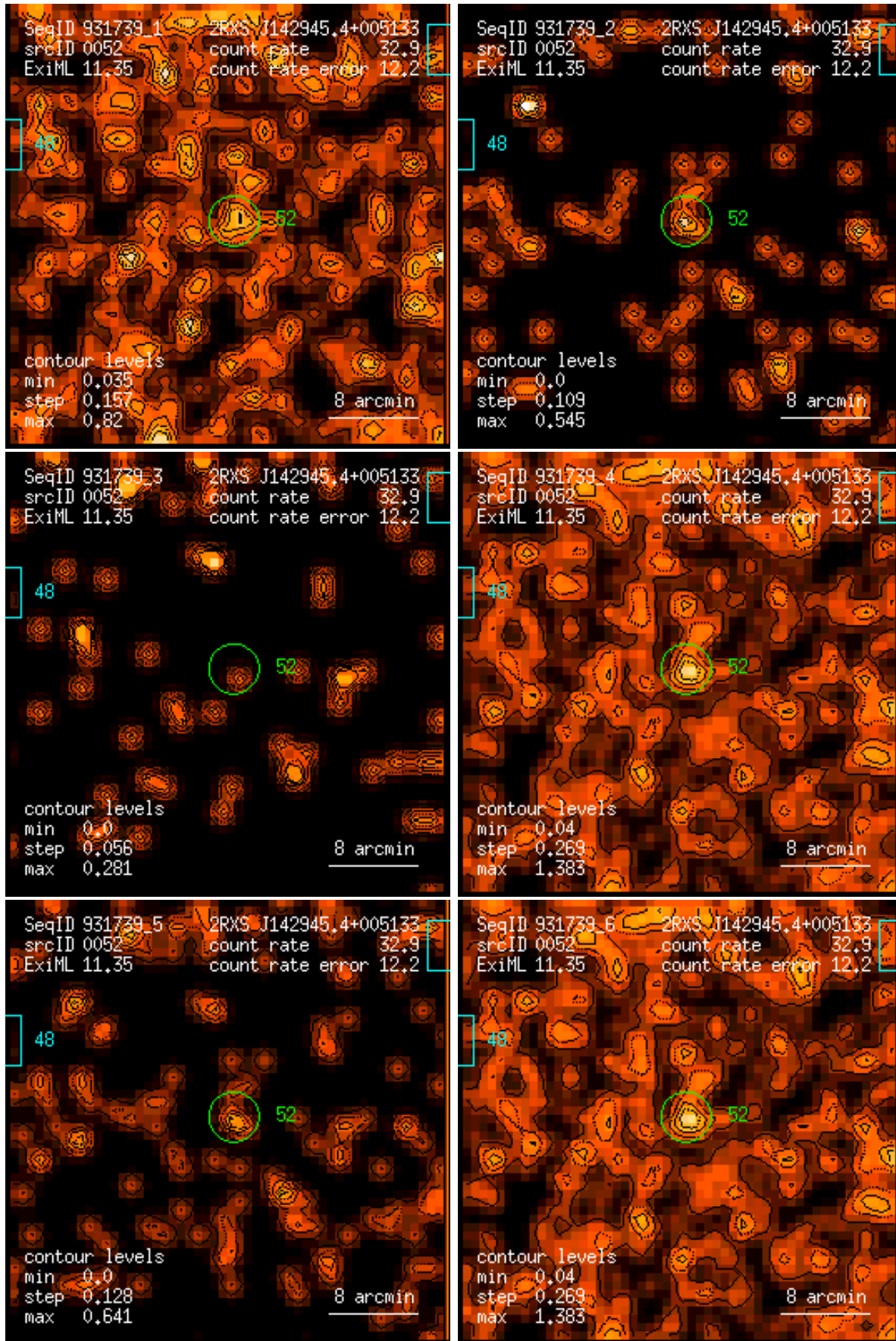
Figure 52: RASS 931739: detection 0052: band rate images, Gaussian filter: (1) PSPC channels 11 – 41, (2) 52 – 90, (3) 91 – 201, (4) 11 – 235, (5) 52 – 201, (6) 11 – 201. Broad band rates in counts/ks. Band rate contour levels in counts/ks/arcmin 2 .
