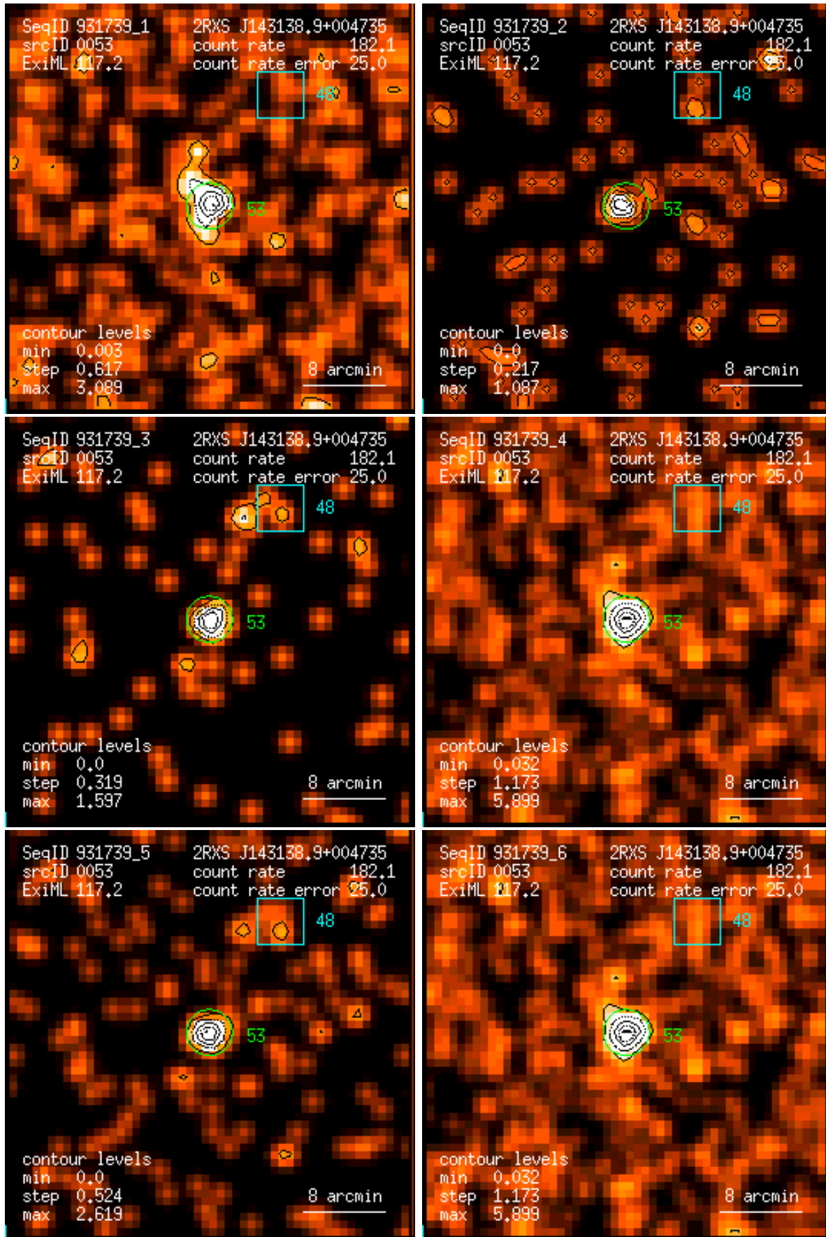
Figure 53: RASS 931739: detection 0053: band rate images, Gaussian filter: (1) PSPC channels 11 – 41, (2) 52 – 90, (3) 91 – 201, (4) 11 – 235, (5) 52 – 201, (6) 11 – 201. Broad band rates in counts/ks. Band rate contour levels in counts/ks/arcmin 2 .
