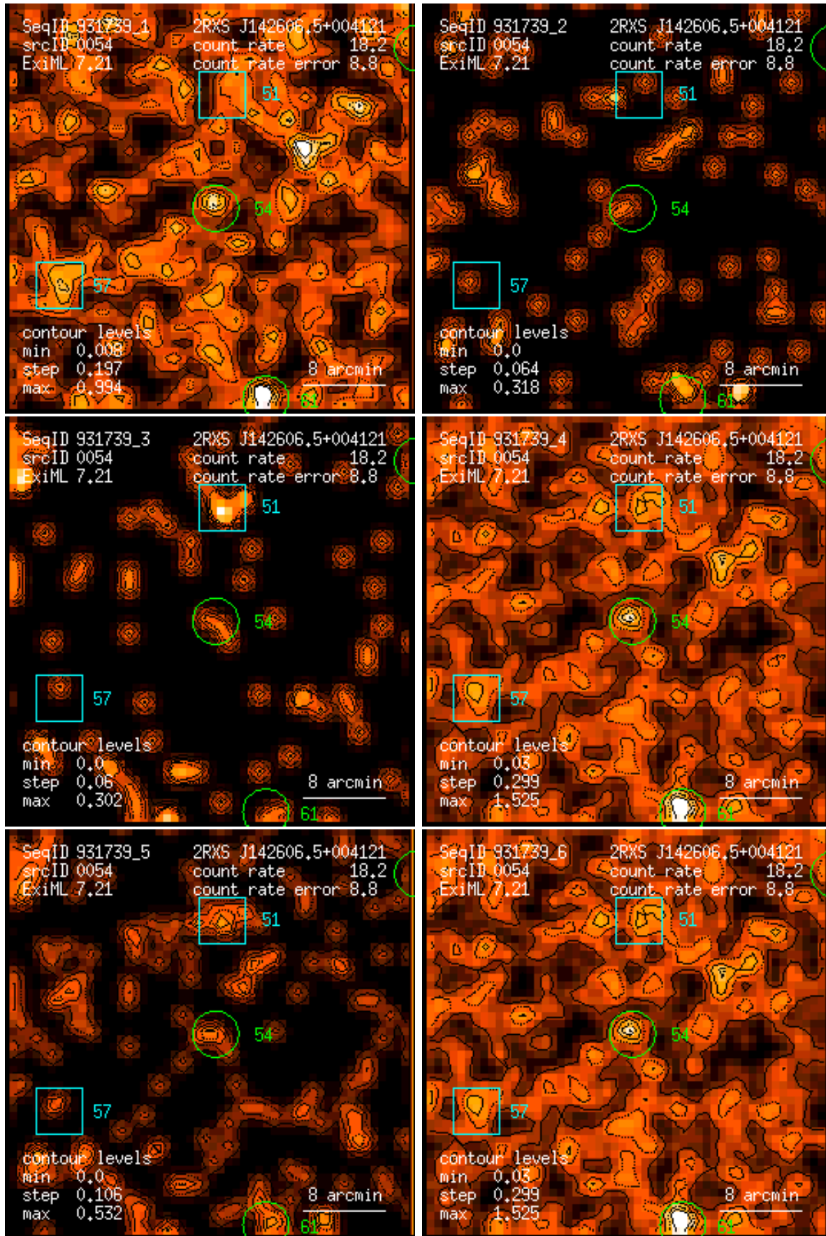
Figure 54: RASS 931739: detection 0054: band rate images, Gaussian filter: (1) PSPC channels 11 – 41, (2) 52 – 90, (3) 91 – 201, (4) 11 – 235, (5) 52 – 201, (6) 11 – 201. Broad band rates in counts/ks. Band rate contour levels in counts/ks/arcmin 2 .
