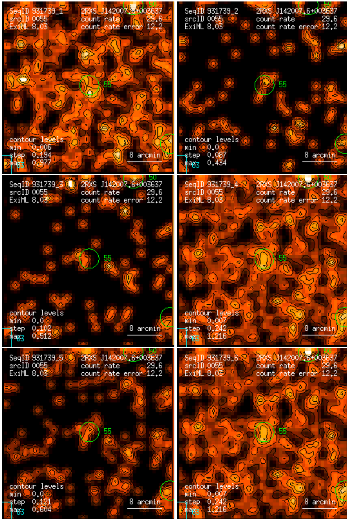
Figure 55: RASS 931739: detection 0055: band rate images, Gaussian filter: (1) PSPC channels 11 – 41, (2) 52 – 90, (3) 91 – 201, (4) 11 – 235, (5) 52 – 201, (6) 11 – 201. Broad band rates in counts/ks. Band rate contour levels in counts/ks/arcmin 2 .
