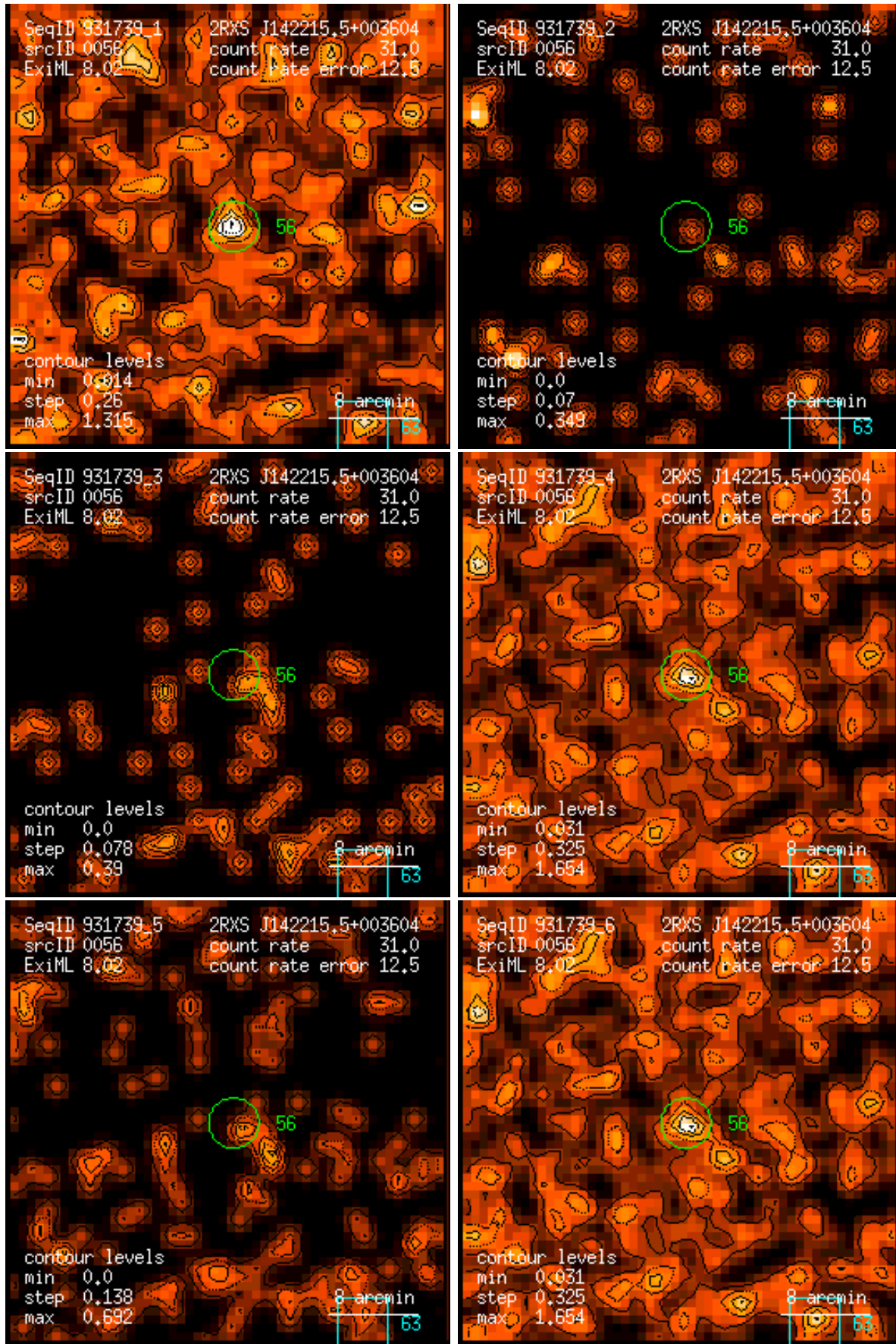
Figure 56: RASS 931739: detection 0056: band rate images, Gaussian filter: (1) PSPC channels 11 – 41, (2) 52 – 90, (3) 91 – 201, (4) 11 – 235, (5) 52 – 201, (6) 11 – 201. Broad band rates in counts/ks. Band rate contour levels in counts/ks/arcmin 2 .
