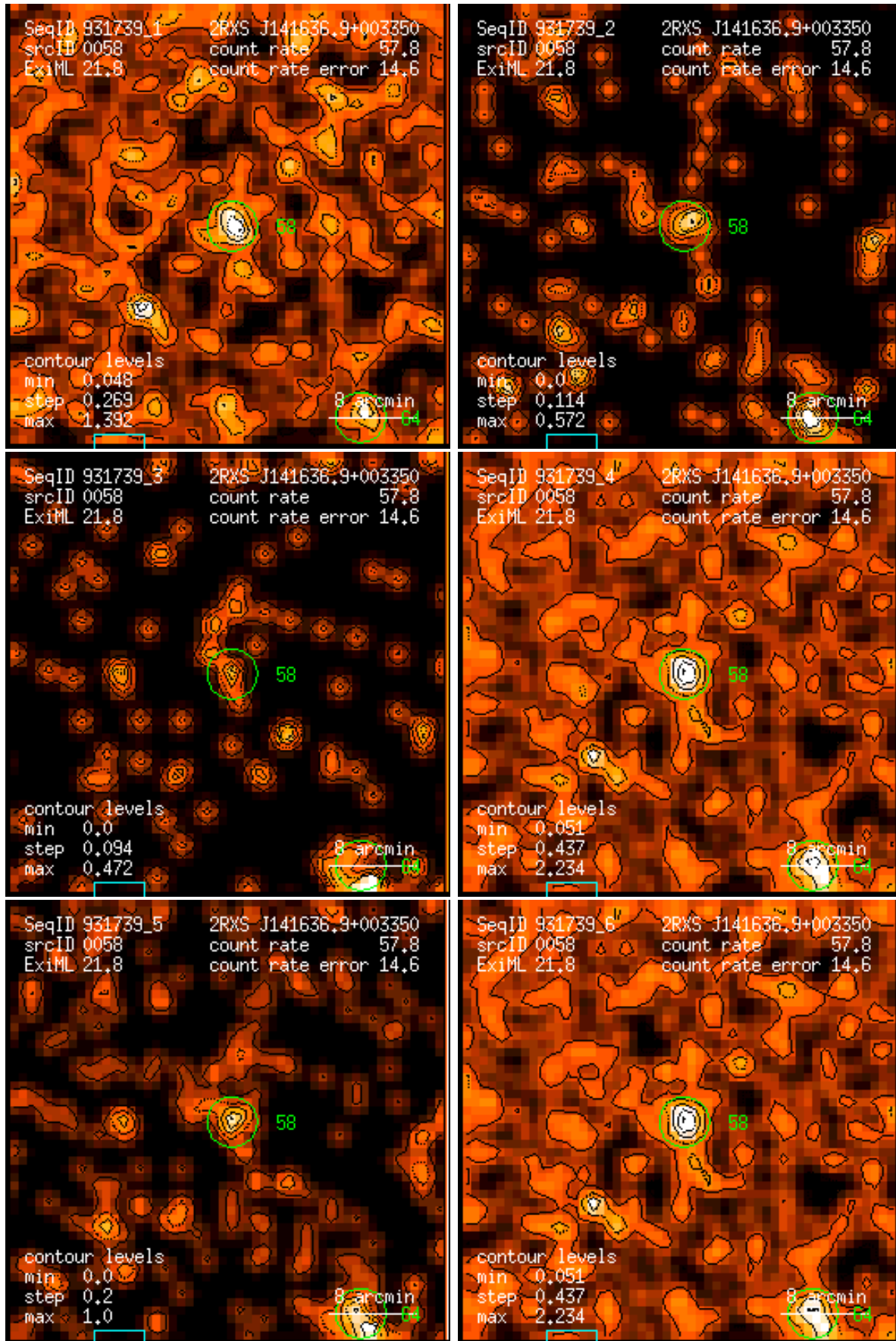
Figure 58: RASS 931739: detection 0058: band rate images, Gaussian filter: (1) PSPC channels 11 – 41, (2) 52 – 90, (3) 91 – 201, (4) 11 – 235, (5) 52 – 201, (6) 11 – 201. Broad band rates in counts/ks. Band rate contour levels in counts/ks/arcmin 2 .
