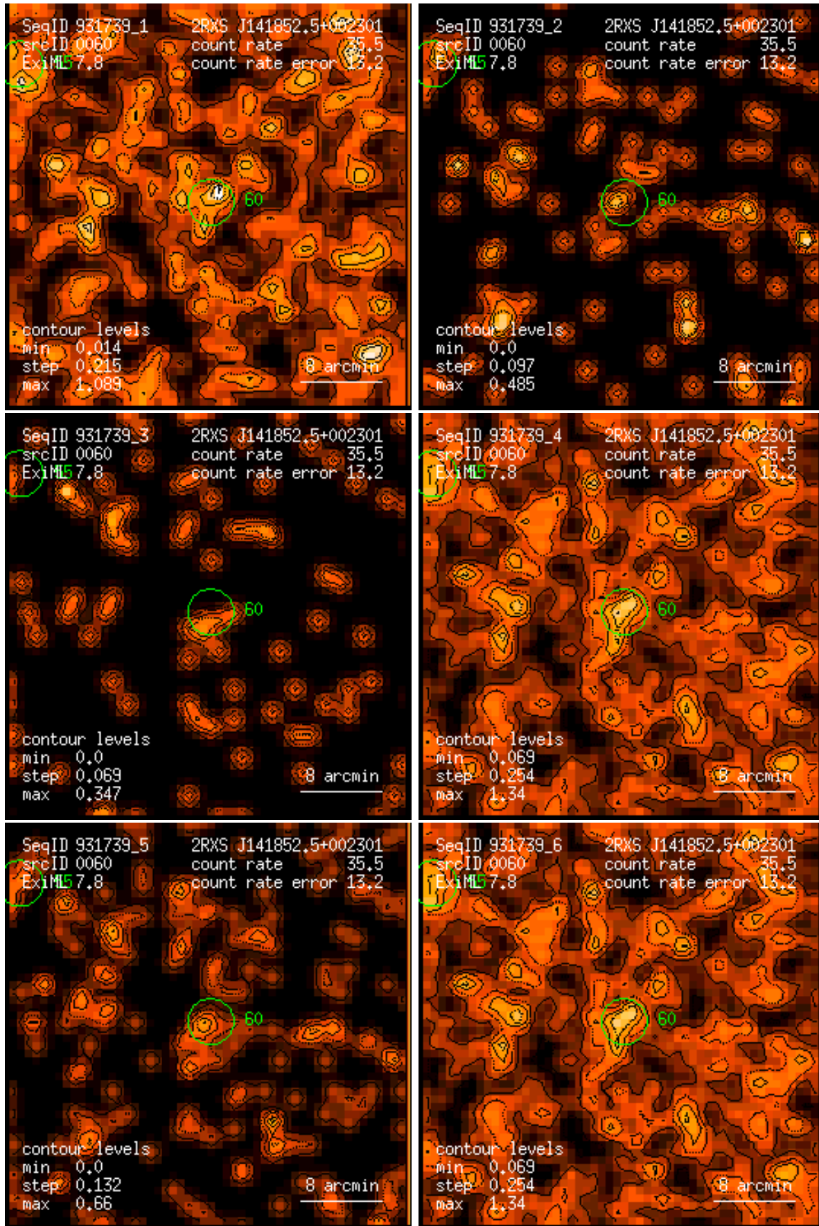
Figure 60: RASS 931739: detection 0060: band rate images, Gaussian filter: (1) PSPC channels 11 – 41, (2) 52 – 90, (3) 91 – 201, (4) 11 – 235, (5) 52 – 201, (6) 11 – 201. Broad band rates in counts/ks. Band rate contour levels in counts/ks/arcmin 2 .
