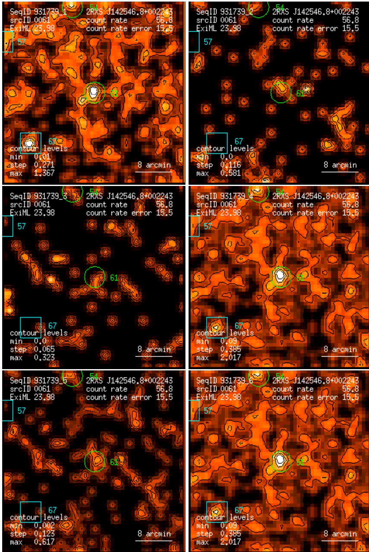
Figure 61: RASS 931739: detection 0061: band rate images, Gaussian filter: (1) PSPC channels 11 – 41, (2) 52 – 90, (3) 91 – 201, (4) 11 – 235, (5) 52 – 201, (6) 11 – 201. Broad band rates in counts/ks. Band rate contour levels in counts/ks/arcmin 2 .
