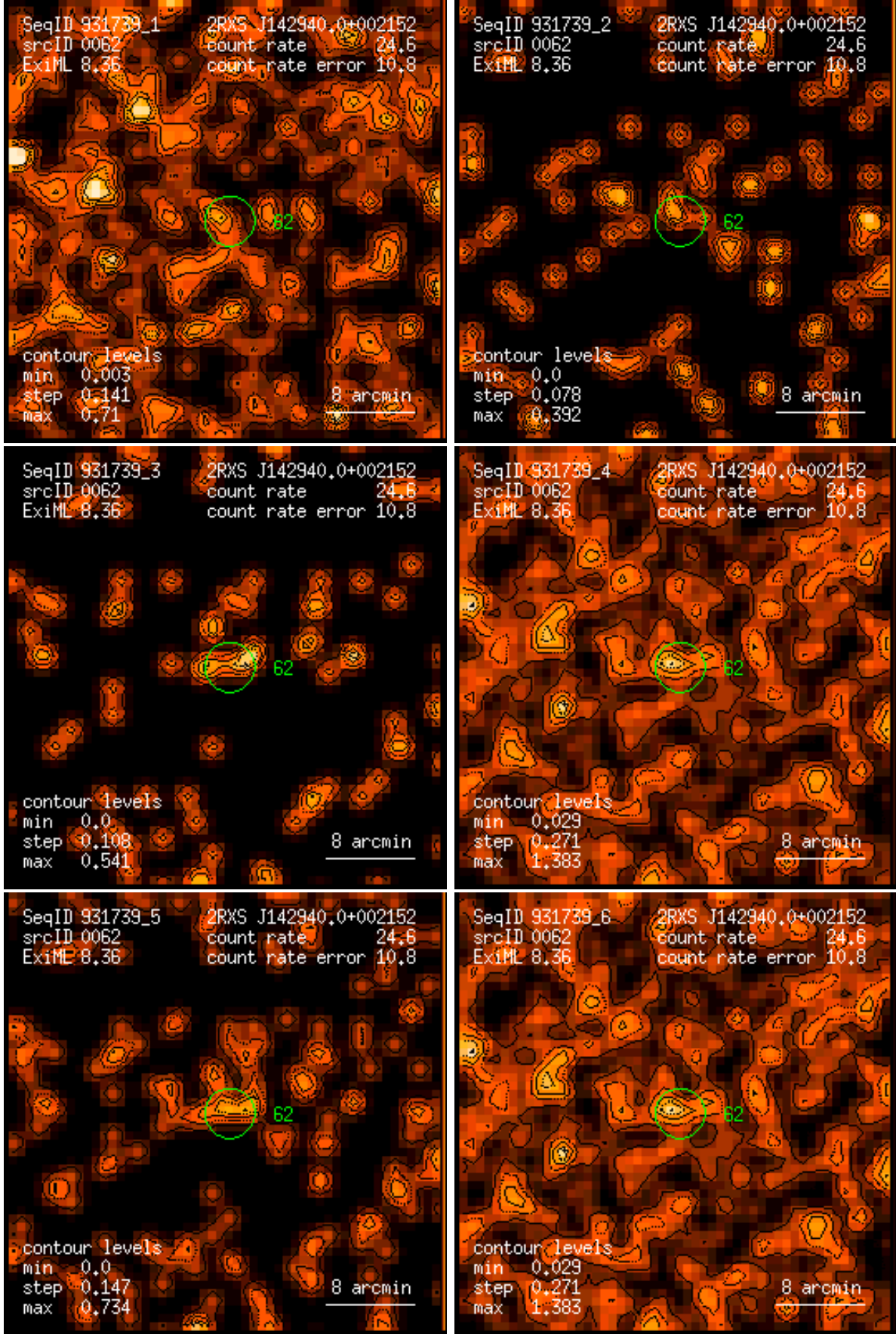
Figure 62: RASS 931739: detection 0062: band rate images, Gaussian filter: (1) PSPC channels 11 – 41, (2) 52 – 90, (3) 91 – 201, (4) 11 – 235, (5) 52 – 201, (6) 11 – 201. Broad band rates in counts/ks. Band rate contour levels in counts/ks/arcmin 2 .
