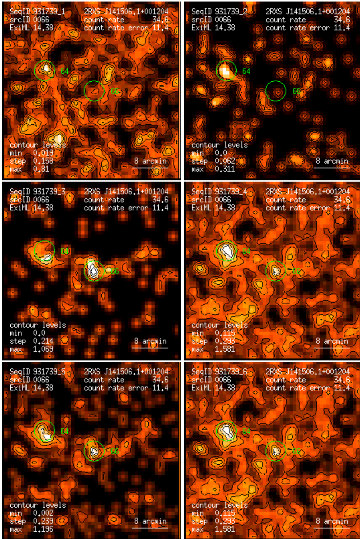
Figure 66: RASS 931739: detection 0066: band rate images, Gaussian filter: (1) PSPC channels 11 – 41, (2) 52 – 90, (3) 91 – 201, (4) 11 – 235, (5) 52 – 201, (6) 11 – 201. Broad band rates in counts/ks. Band rate contour levels in counts/ks/arcmin 2 .
