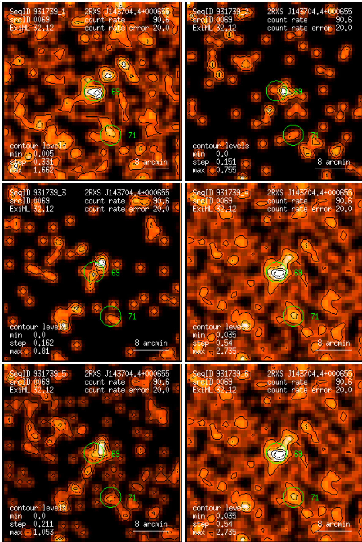
Figure 69: RASS 931739: detection 0069: band rate images, Gaussian filter: (1) PSPC channels 11 – 41, (2) 52 – 90, (3) 91 – 201, (4) 11 – 235, (5) 52 – 201, (6) 11 – 201. Broad band rates in counts/ks. Band rate contour levels in counts/ks/arcmin 2 .
