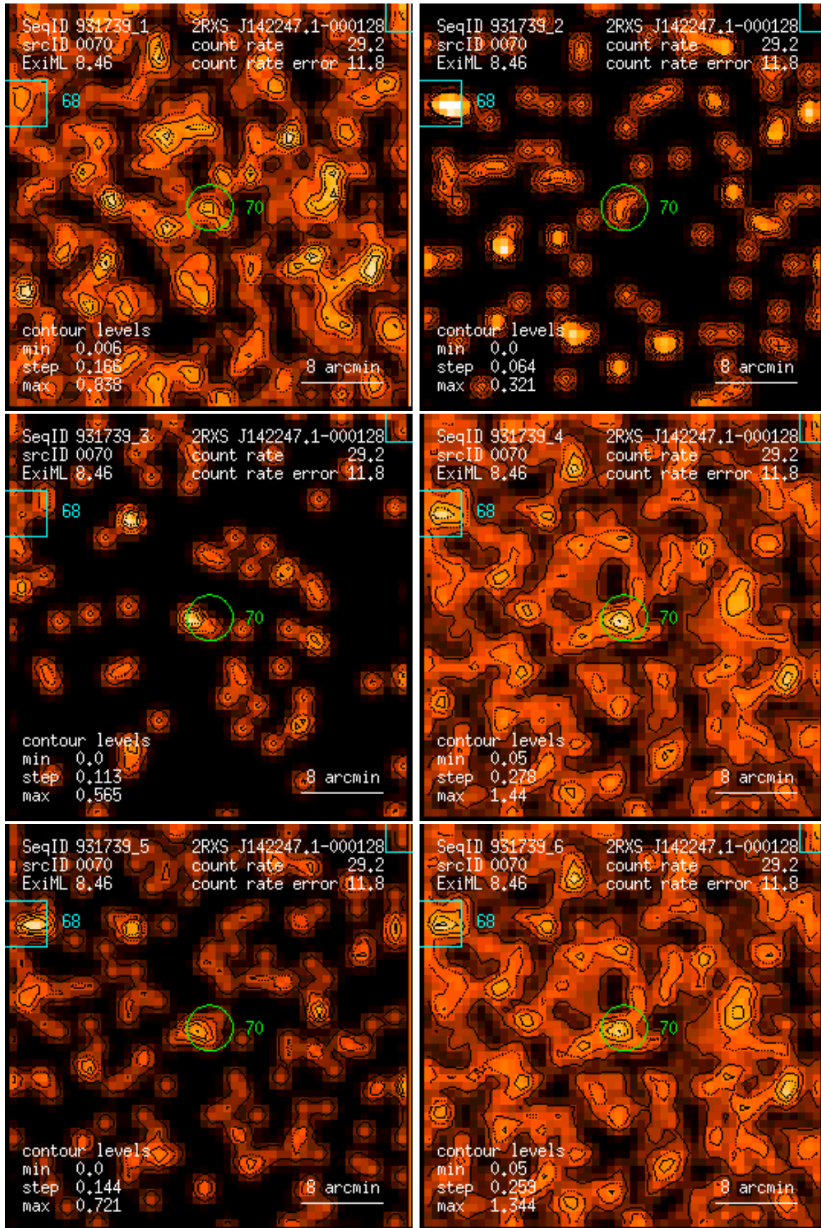
Figure 70: RASS 931739: detection 0070: band rate images, Gaussian filter: (1) PSPC channels 11 – 41, (2) 52 – 90, (3) 91 – 201, (4) 11 – 235, (5) 52 – 201, (6) 11 – 201. Broad band rates in counts/ks. Band rate contour levels in counts/ks/arcmin 2 .
