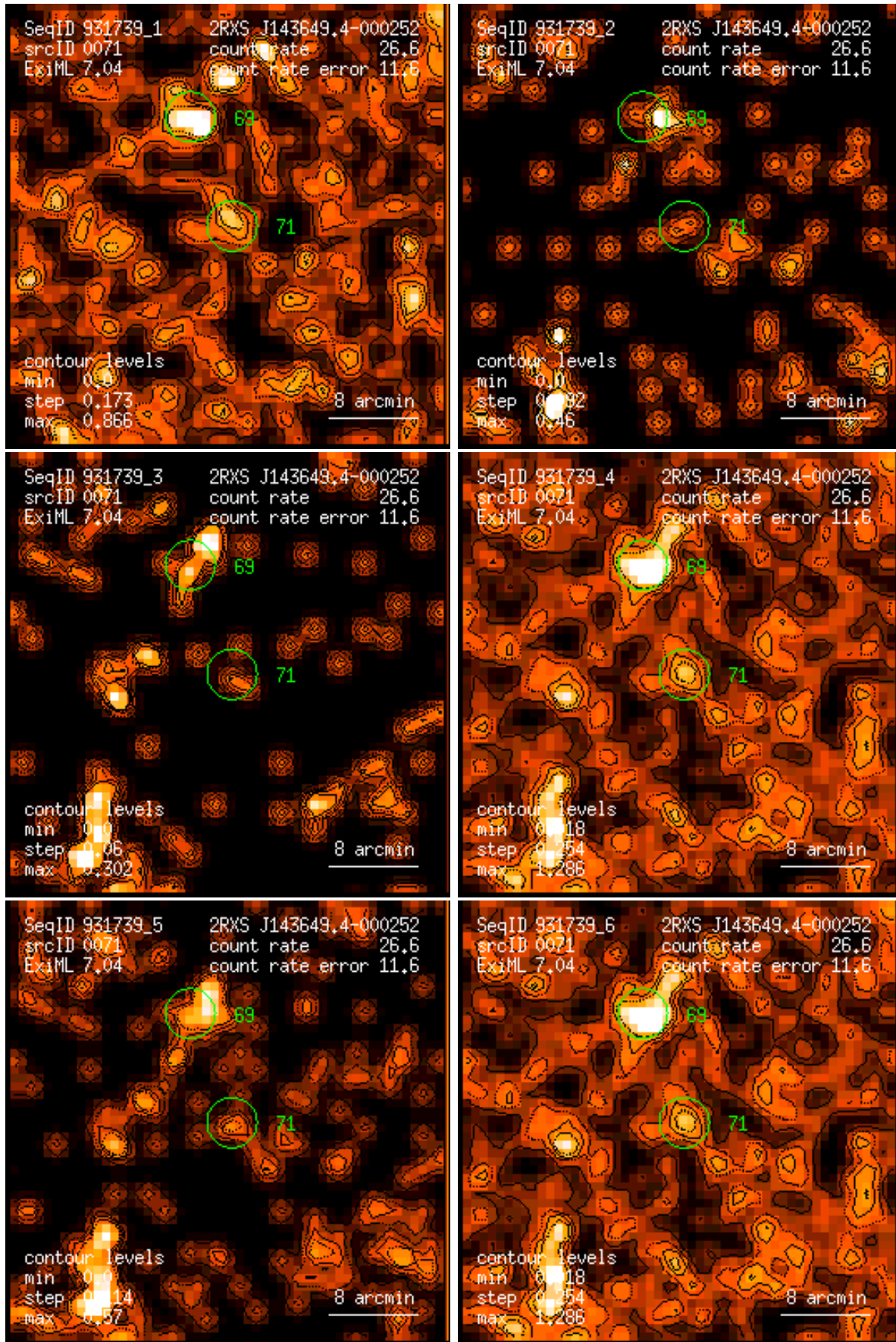
Figure 71: RASS 931739: detection 0071: band rate images, Gaussian filter: (1) PSPC channels 11 – 41, (2) 52 – 90, (3) 91 – 201, (4) 11 – 235, (5) 52 – 201, (6) 11 – 201. Broad band rates in counts/ks. Band rate contour levels in counts/ks/arcmin 2 .
