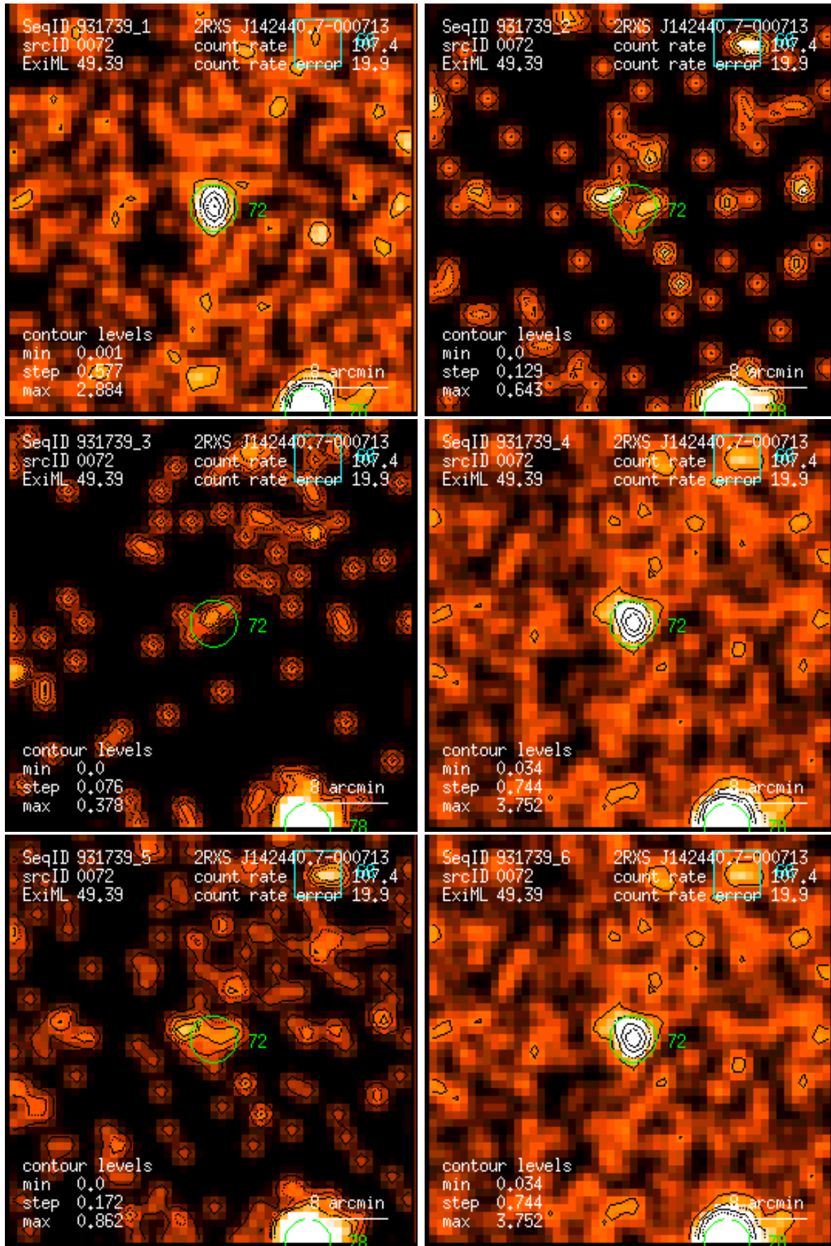
Figure 72: RASS 931739: detection 0072: band rate images, Gaussian filter: (1) PSPC channels 11 – 41, (2) 52 – 90, (3) 91 – 201, (4) 11 – 235, (5) 52 – 201, (6) 11 – 201. Broad band rates in counts/ks. Band rate contour levels in counts/ks/arcmin 2 .
