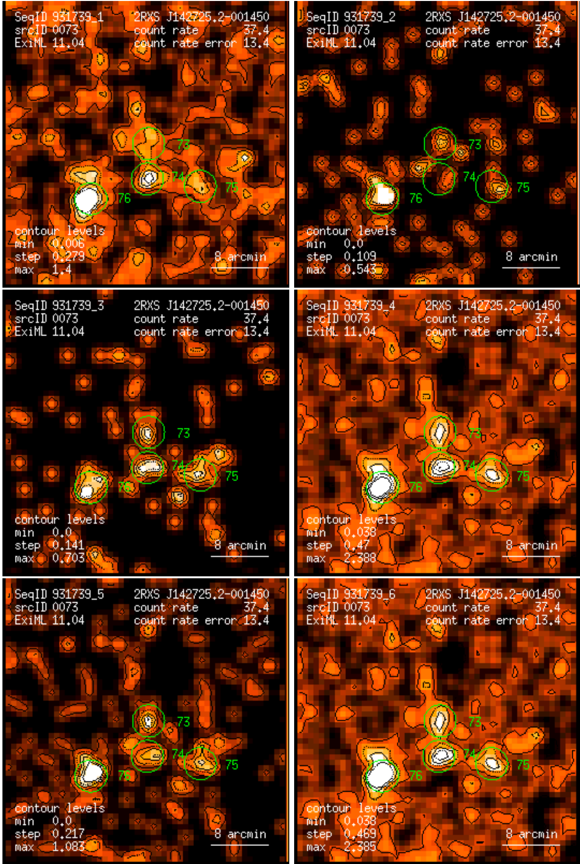
Figure 73: RASS 931739: detection 0073: band rate images, Gaussian filter: (1) PSPC channels 11 – 41, (2) 52 – 90, (3) 91 – 201, (4) 11 – 235, (5) 52 – 201, (6) 11 – 201. Broad band rates in counts/ks. Band rate contour levels in counts/ks/arcmin 2 .
