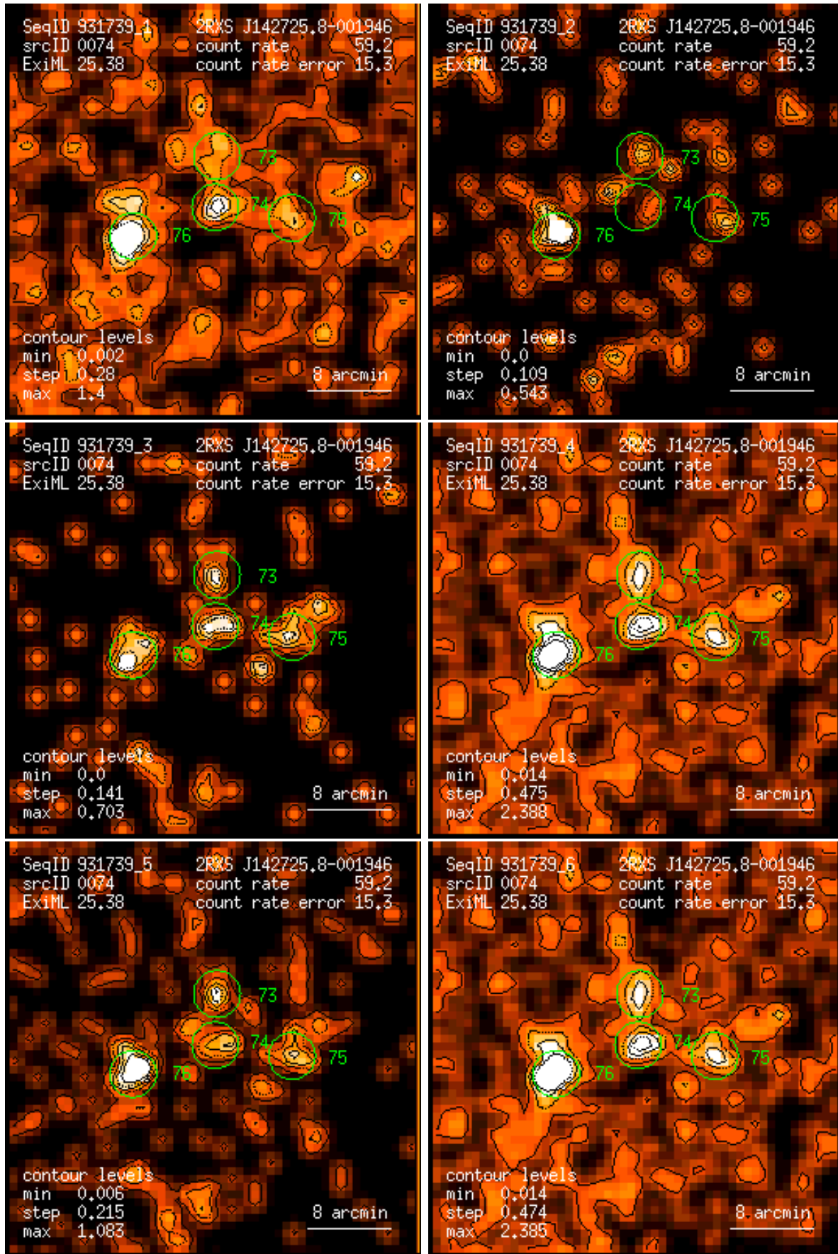
Figure 74: RASS 931739: detection 0074: band rate images, Gaussian filter: (1) PSPC channels 11 – 41, (2) 52 – 90, (3) 91 – 201, (4) 11 – 235, (5) 52 – 201, (6) 11 – 201. Broad band rates in counts/ks. Band rate contour levels in counts/ks/arcmin 2 .
