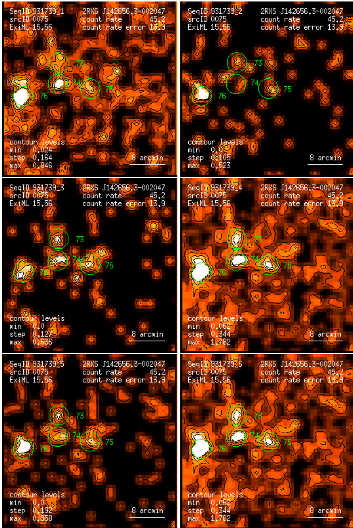
Figure 75: RASS 931739: detection 0075: band rate images, Gaussian filter: (1) PSPC channels 11 – 41, (2) 52 – 90, (3) 91 – 201, (4) 11 – 235, (5) 52 – 201, (6) 11 – 201. Broad band rates in counts/ks. Band rate contour levels in counts/ks/arcmin 2 .
