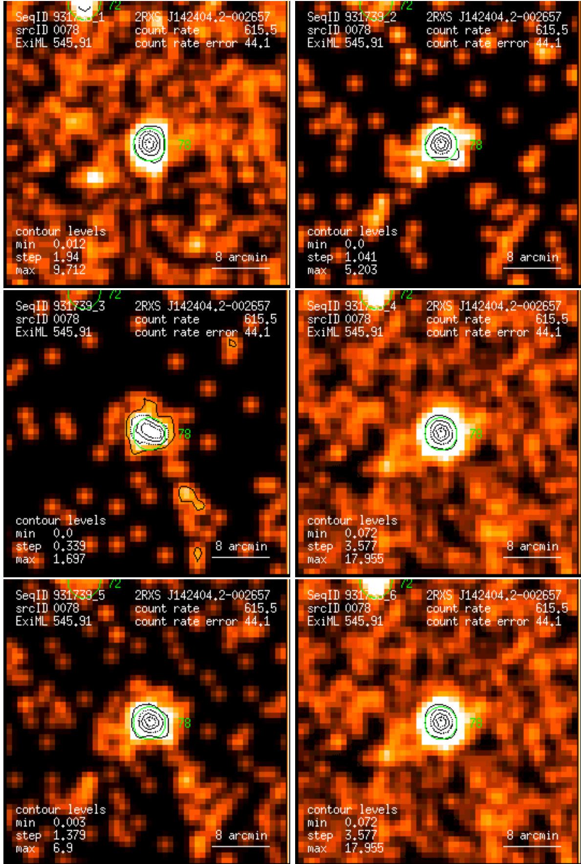
Figure 78: RASS 931739: detection 0078: band rate images, Gaussian filter: (1) PSPC channels 11 – 41, (2) 52 – 90, (3) 91 – 201, (4) 11 – 235, (5) 52 – 201, (6) 11 – 201. Broad band rates in counts/ks. Band rate contour levels in counts/ks/arcmin 2 .
