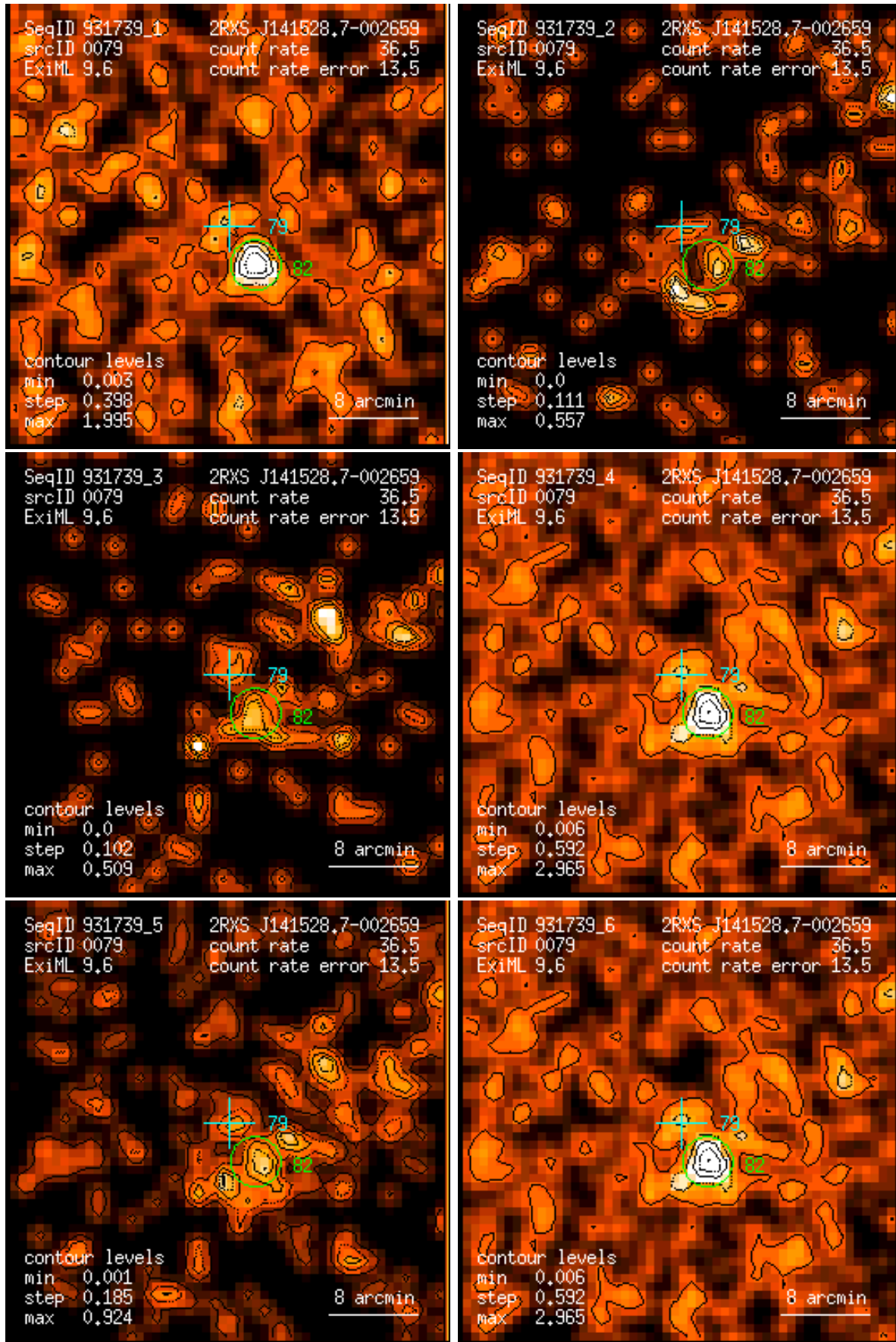
Figure 79: RASS 931739: detection 0079: band rate images, Gaussian filter: (1) PSPC channels 11 – 41, (2) 52 – 90, (3) 91 – 201, (4) 11 – 235, (5) 52 – 201, (6) 11 – 201. Broad band rates in counts/ks. Band rate contour levels in counts/ks/arcmin 2 .
