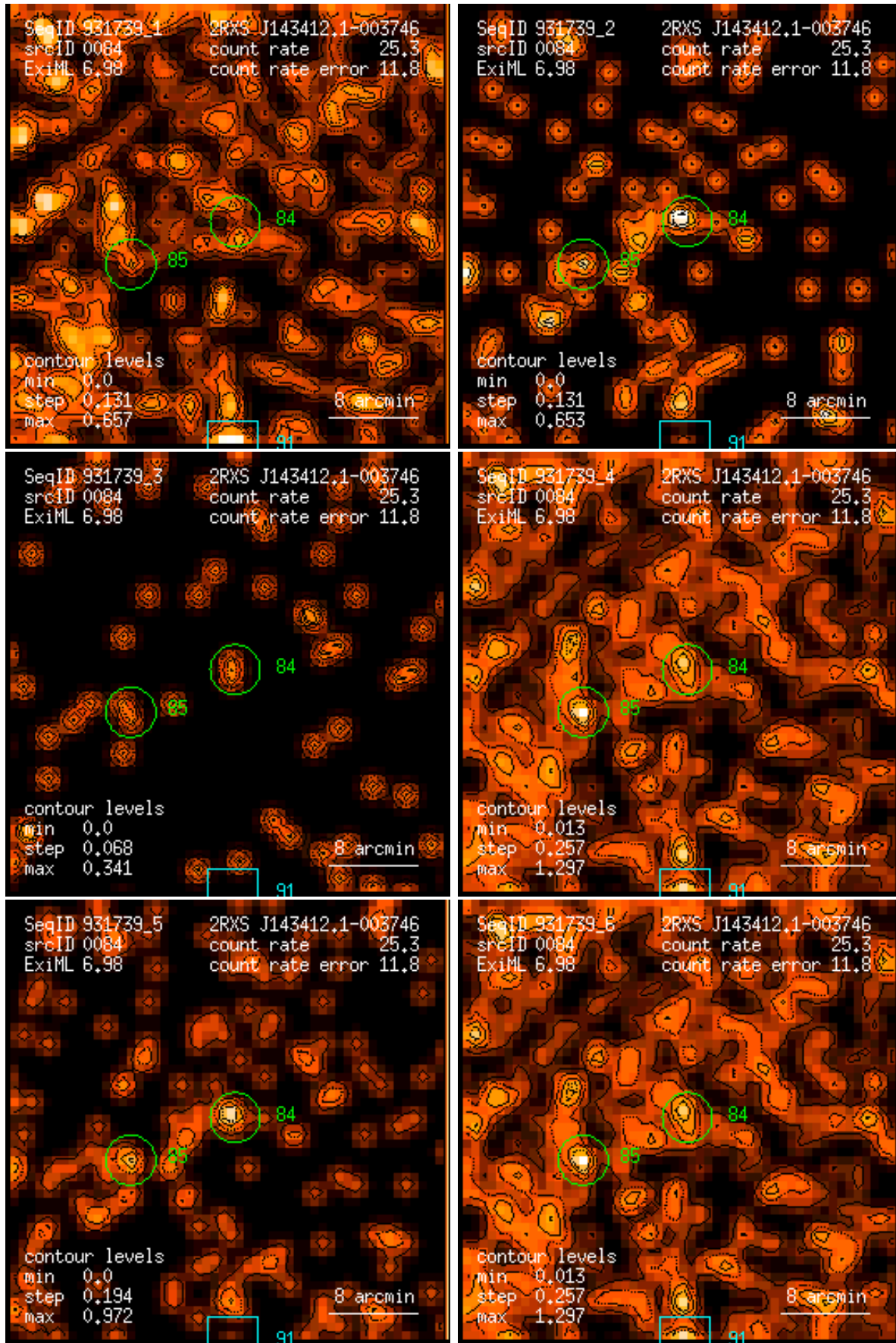
Figure 84: RASS 931739: detection 0084: band rate images, Gaussian filter: (1) PSPC channels 11 – 41, (2) 52 – 90, (3) 91 – 201, (4) 11 – 235, (5) 52 – 201, (6) 11 – 201. Broad band rates in counts/ks. Band rate contour levels in counts/ks/arcmin 2 .
