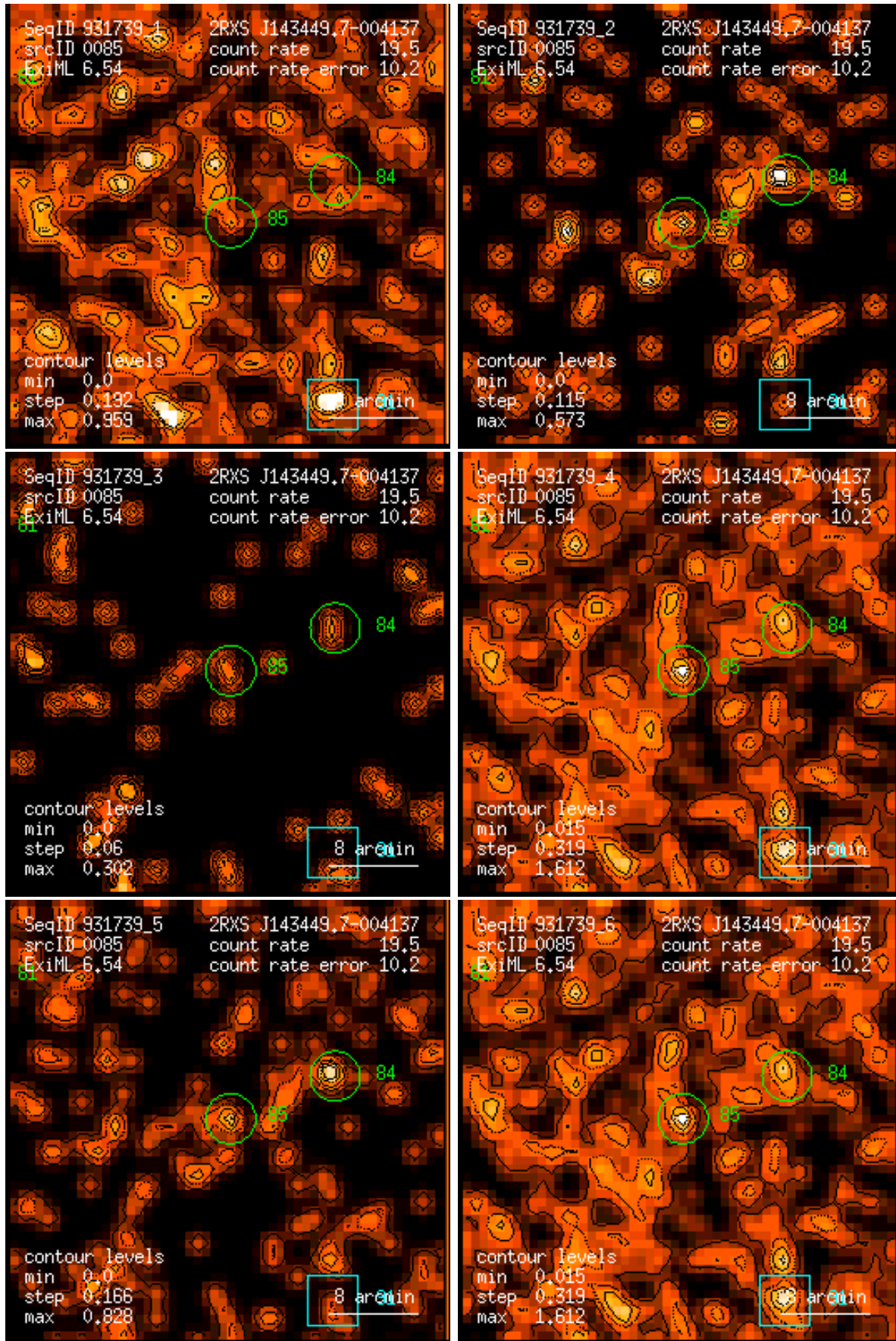
Figure 85: RASS 931739: detection 0085: band rate images, Gaussian filter: (1) PSPC channels 11 – 41, (2) 52 – 90, (3) 91 – 201, (4) 11 – 235, (5) 52 – 201, (6) 11 – 201. Broad band rates in counts/ks. Band rate contour levels in counts/ks/arcmin 2 .
