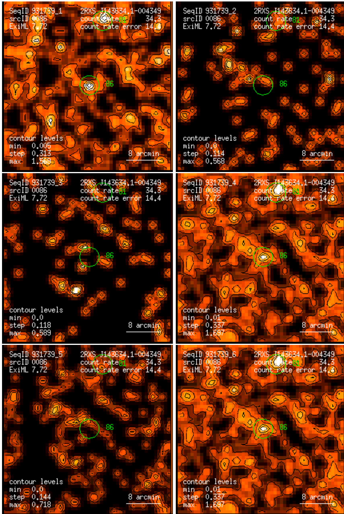
Figure 86: RASS 931739: detection 0086: band rate images, Gaussian filter: (1) PSPC channels 11 – 41, (2) 52 – 90, (3) 91 – 201, (4) 11 – 235, (5) 52 – 201, (6) 11 – 201. Broad band rates in counts/ks. Band rate contour levels in counts/ks/arcmin 2 .
