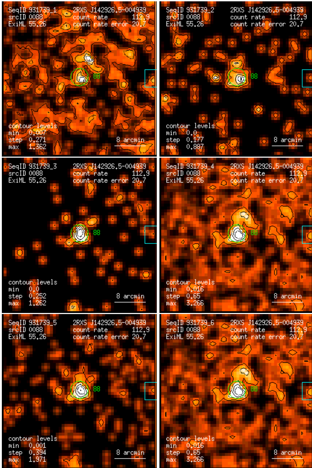
Figure 88: RASS 931739: detection 0088: band rate images, Gaussian filter: (1) PSPC channels 11 – 41, (2) 52 – 90, (3) 91 – 201, (4) 11 – 235, (5) 52 – 201, (6) 11 – 201. Broad band rates in counts/ks. Band rate contour levels in counts/ks/arcmin 2 .
