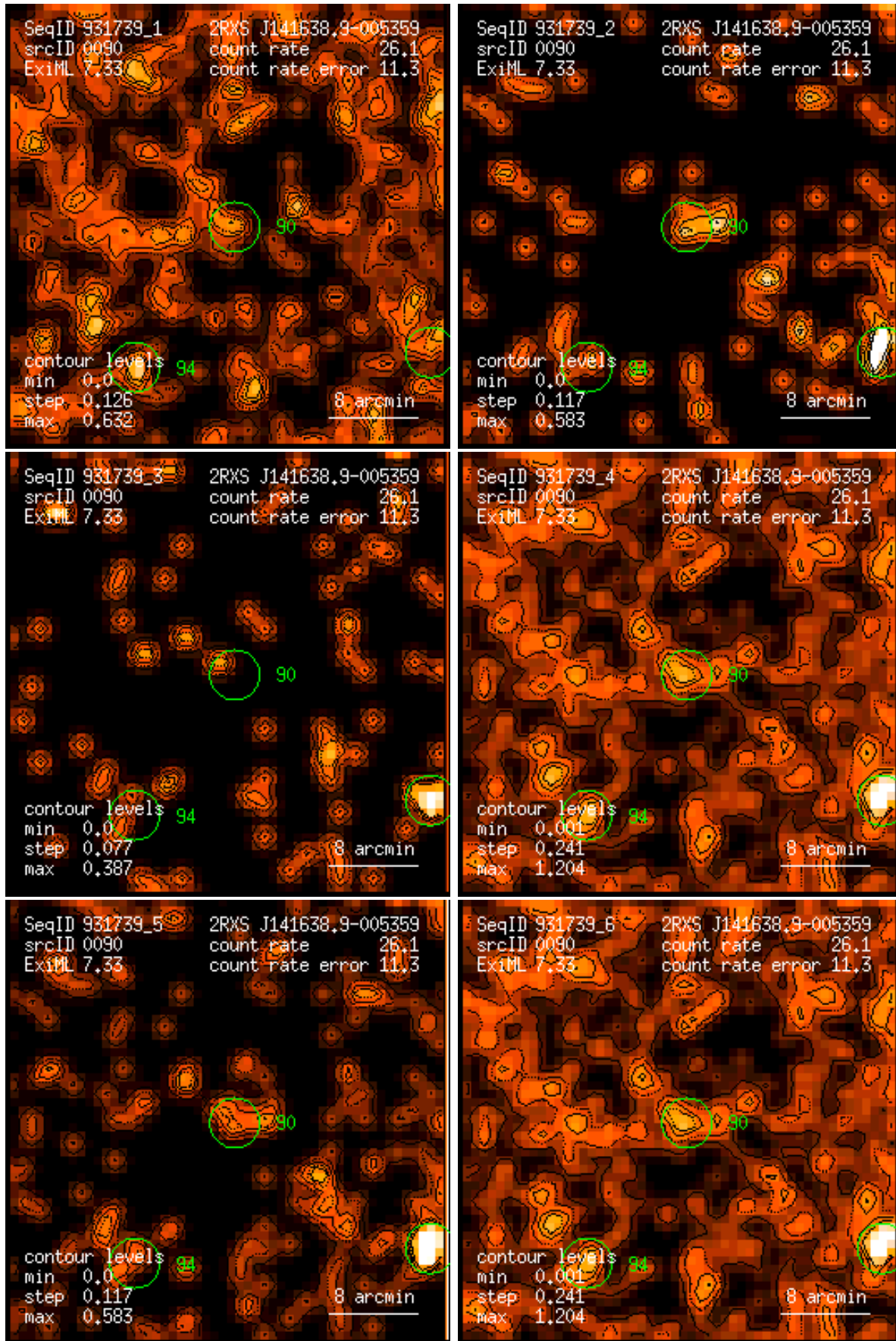
Figure 90: RASS 931739: detection 0090: band rate images, Gaussian filter: (1) PSPC channels 11 – 41, (2) 52 – 90, (3) 91 – 201, (4) 11 – 235, (5) 52 – 201, (6) 11 – 201. Broad band rates in counts/ks. Band rate contour levels in counts/ks/arcmin 2 .
