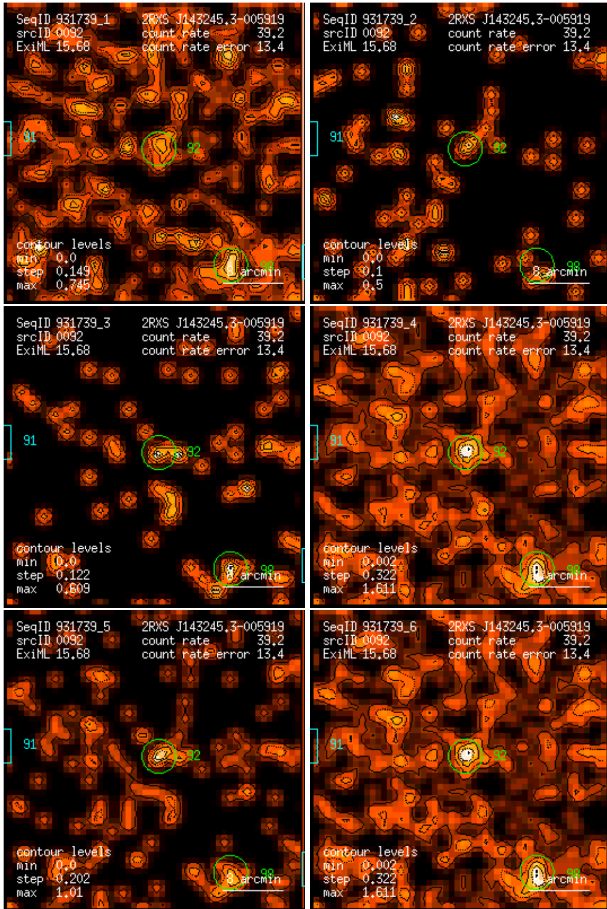
Figure 92: RASS 931739: detection 0092: band rate images, Gaussian filter: (1) PSPC channels 11 – 41, (2) 52 – 90, (3) 91 – 201, (4) 11 – 235, (5) 52 – 201, (6) 11 – 201. Broad band rates in counts/ks. Band rate contour levels in counts/ks/arcmin 2 .
