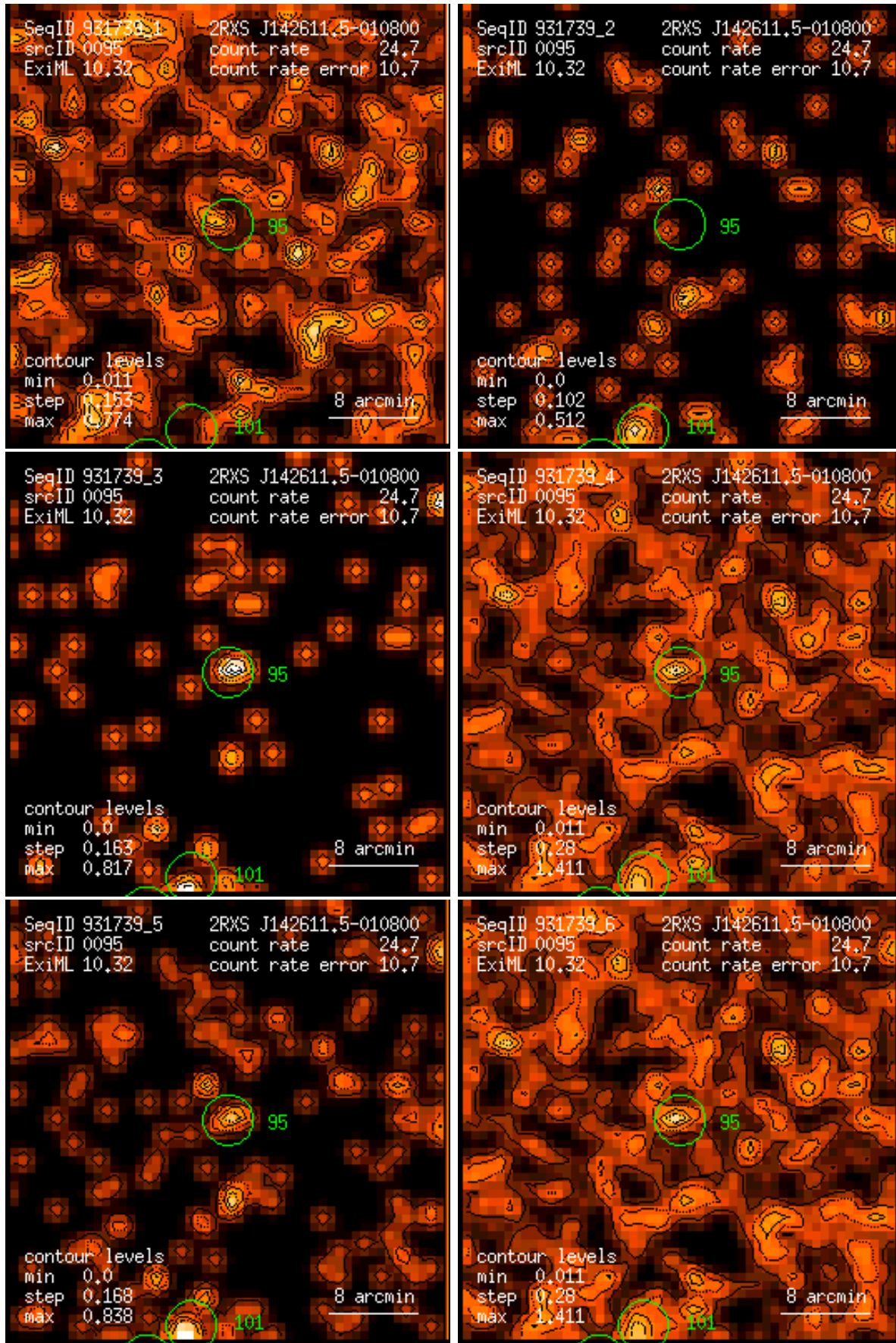
Figure 95: RASS 931739: detection 0095: band rate images, Gaussian filter: (1) PSPC channels 11 – 41, (2) 52 – 90, (3) 91 – 201, (4) 11 – 235, (5) 52 – 201, (6) 11 – 201. Broad band rates in counts/ks. Band rate contour levels in counts/ks/arcmin 2 .
