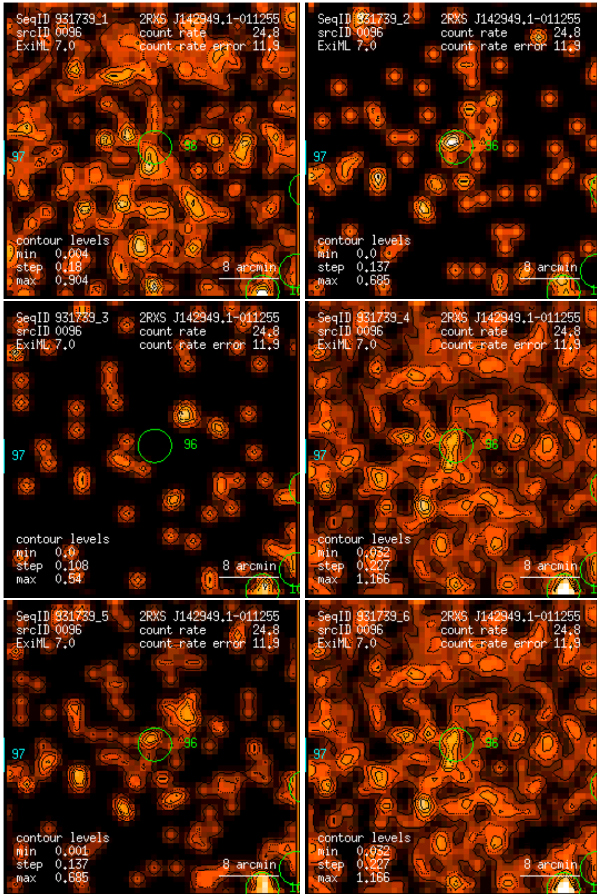
Figure 96: RASS 931739: detection 0096: band rate images, Gaussian filter: (1) PSPC channels 11 – 41, (2) 52 – 90, (3) 91 – 201, (4) 11 – 235, (5) 52 – 201, (6) 11 – 201. Broad band rates in counts/ks. Band rate contour levels in counts/ks/arcmin 2 .
