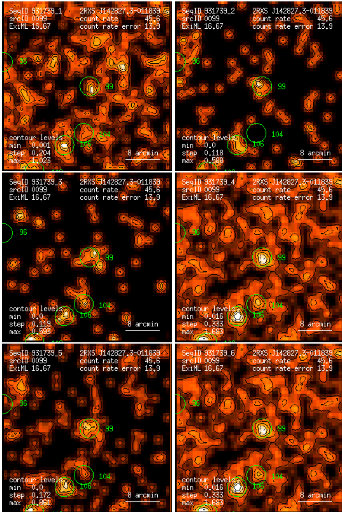
Figure 99: RASS 931739: detection 0099: band rate images, Gaussian filter: (1) PSPC channels 11 – 41, (2) 52 – 90, (3) 91 – 201, (4) 11 – 235, (5) 52 – 201, (6) 11 – 201. Broad band rates in counts/ks. Band rate contour levels in counts/ks/arcmin 2 .
