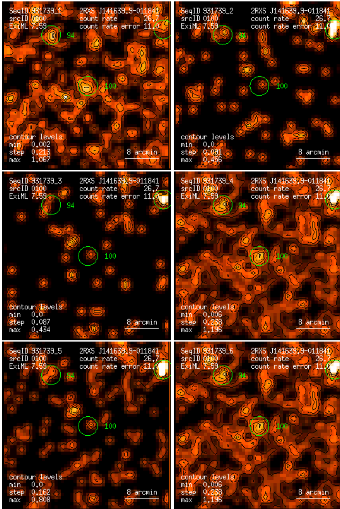
Figure 100: RASS 931739: detection 0100: band rate images, Gaussian filter: (1) PSPC channels 11 – 41, (2) 52 – 90, (3) 91 – 201, (4) 11 – 235, (5) 52 – 201, (6) 11 – 201. Broad band rates in counts/ks. Band rate contour levels in counts/ks/arcmin 2 .
